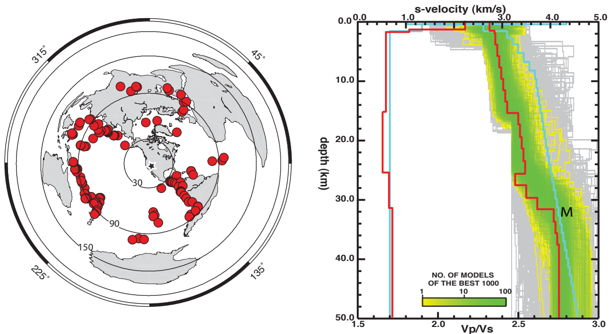
Figure 6a (left): >200 teleseismic events (mb > 5.5 and 30^\circ \leq epicentral distance \leq 110^\circ ) recorded in 8-month "NV-Earthscope-04" deployment (see Figure 1 for location).
