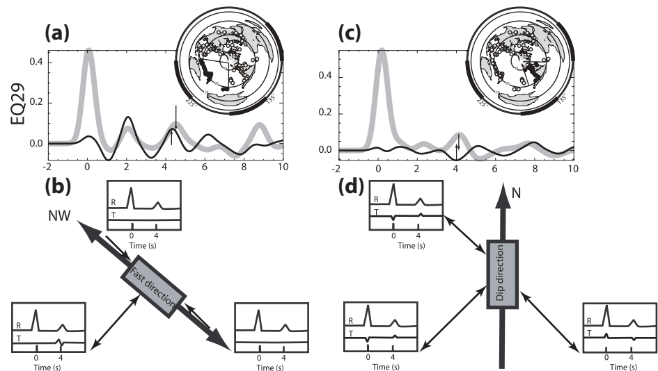
Figure 8: Crustal anisotropy determination from analyses of “NV-FlexArray-04”.
