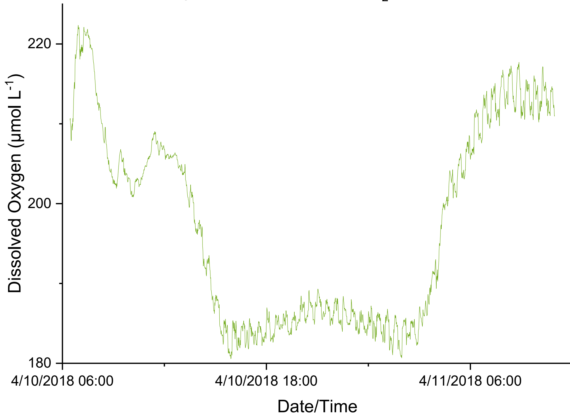
Middle Brother Lagoon BEAMS dissolved O 2 SBE37 - 2018 - 30 hours
