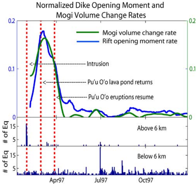
Fig. 10 Normalized time evolving of rift opening moment rate, normalized by a maximum of 7.8 m/year, and magma chamber inflation rate, normalized by a maximum volume change rate of 0.02 \text{ km}^3/\text{year} . The red dotted lines show the time of the intrusion, the refilled lava pond at Pu'u 'Ō'ō, and the time eruptions resumed there. Both rates sharply peak just after the lava pond returns to Pu'u 'Ō'ō. Histograms below, are the number of earthquakes per day above 6 km in the middle frame and below 6 km in the lower frame
