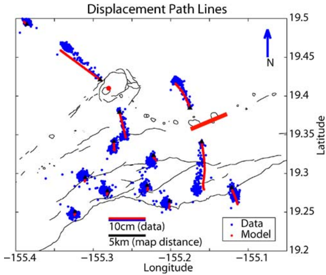
Fig. 6 Displacement pathlines of the ERZ continuous GPS stations for 290 days following the 30 January 1997 intrusion. The data are shown in blue and the model in red. The time series start at the black triangle
