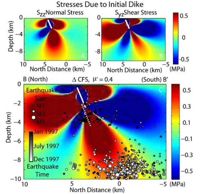
Fig. 11 Stresses due to initial dike. a Vertical normal stresses due to initial dike. b Shear stresses due to initial dike. c Change in Coulomb failure stress on horizontal planes due to the initial 30 January 1997 dike intrusion. Warmer colors are encouraged to slip by the stress change and cooler colors discouraged. The white line shows the location of the 30 January 1997 dike. Relocated south flank earthquakes are also plotted with blacker circles indicating earthquakes that occurred early in the year; the whiter circles occurred later in the year. The size of the circle indicates the magnitude of the event
