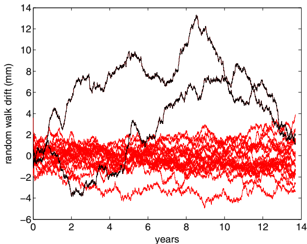
Fig. 7 Kalman filter output of random walk components for synthetic time series. 18 times series have random walk with \tau = 0.3 \text{ mm/year}^{0.5} (red), while 2 time series have random with \tau = 3.0 \text{ mm/year}^{0.5} (black). The anomalous time series are easily identified
