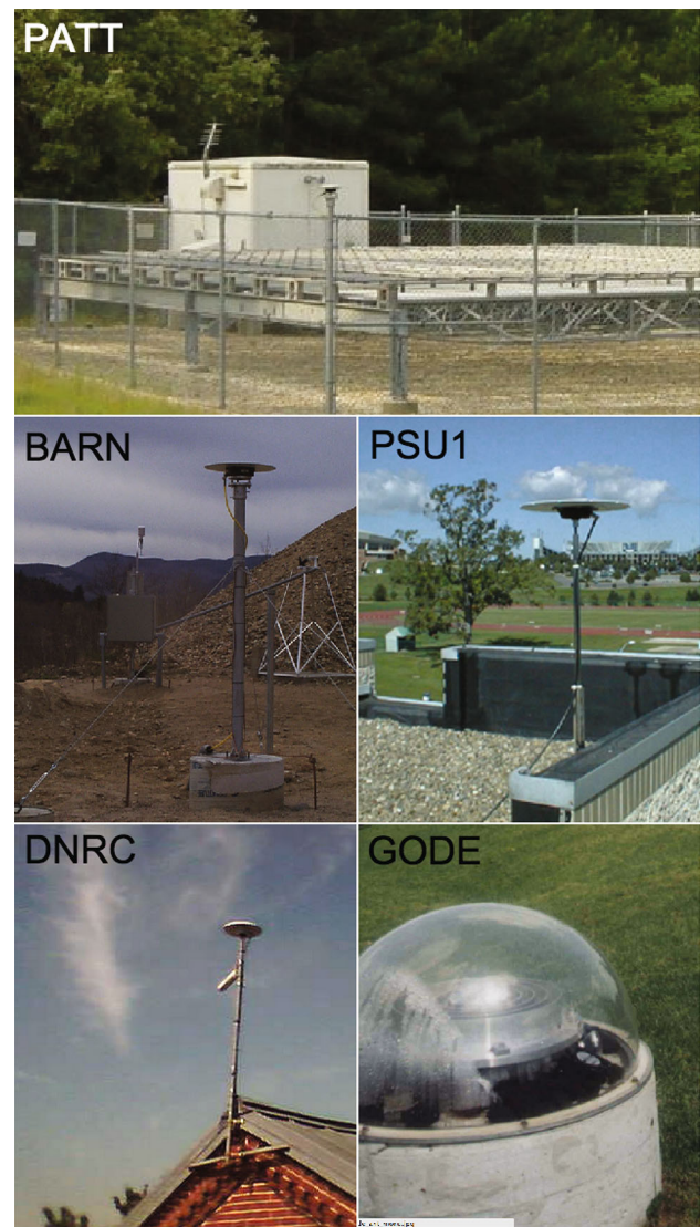
Fig. 12 Examples of station monuments ( http://geodesy.noaa.gov/CORS/ , http://www.profiler.noaa.gov/npn/ ). PATT is located on the corner of a chain link fence. DNRC and PSU1 are installed on metal masts on top of buildings. BARN's antenna is located on a metal mast in a concrete base. GODE is installed on a concrete pillar drilled into the ground
