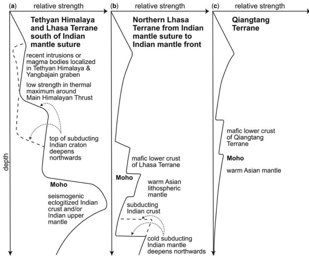
Fig. 7. Cartoons of inferred relative strength–depth profiles for Tibet at about 90^{\circ}\text{E} . The competing effects of increasing temperature with depth and compositional variability (generally more mafic at depth) allow multiple weak channels in the lithosphere. (a) In the Tethyan Himalaya and southern Lhasa terrane the greatest lithospheric strength is likely in the seismogenic upper mantle. Dashed lines represent laterally variable conditions. (b) In the northern Lhasa terrane north of the Indian mantle suture it is uncertain whether the upper crust or upper mantle is stronger, but the weakest zone is probably at the base of the middle crust. (c) In the central and eastern Qiangtang terrane the only significant lithospheric strength is probably in the brittle upper crust; west of c. 85^{\circ}\text{E} the mantle may become somewhat colder and stronger.
