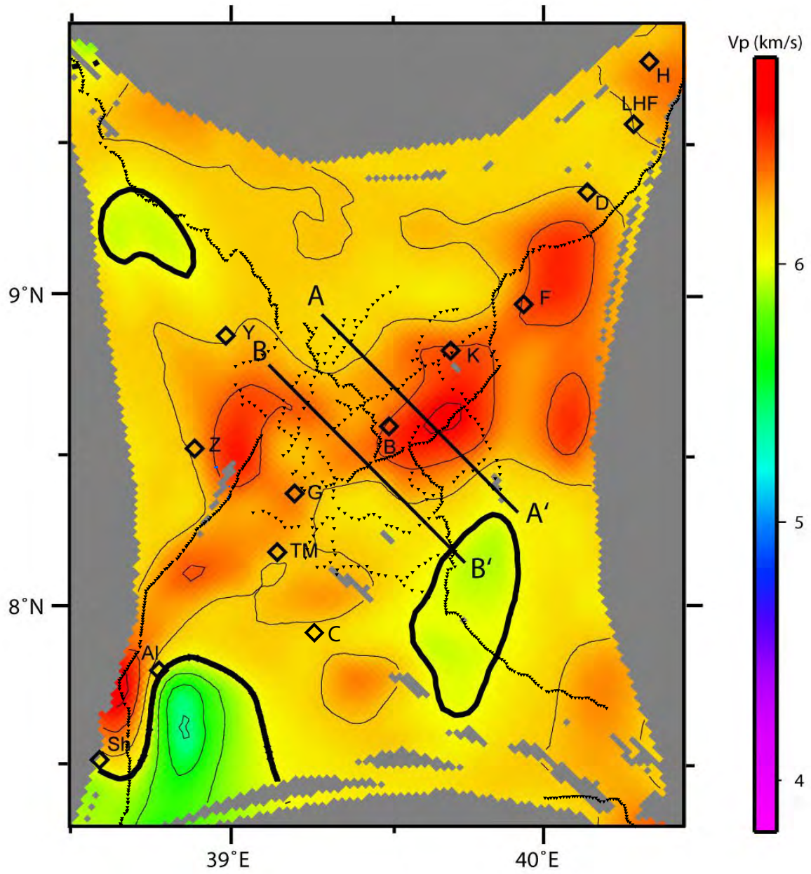
(a) Depth slice at 10 km beneath the NMER
