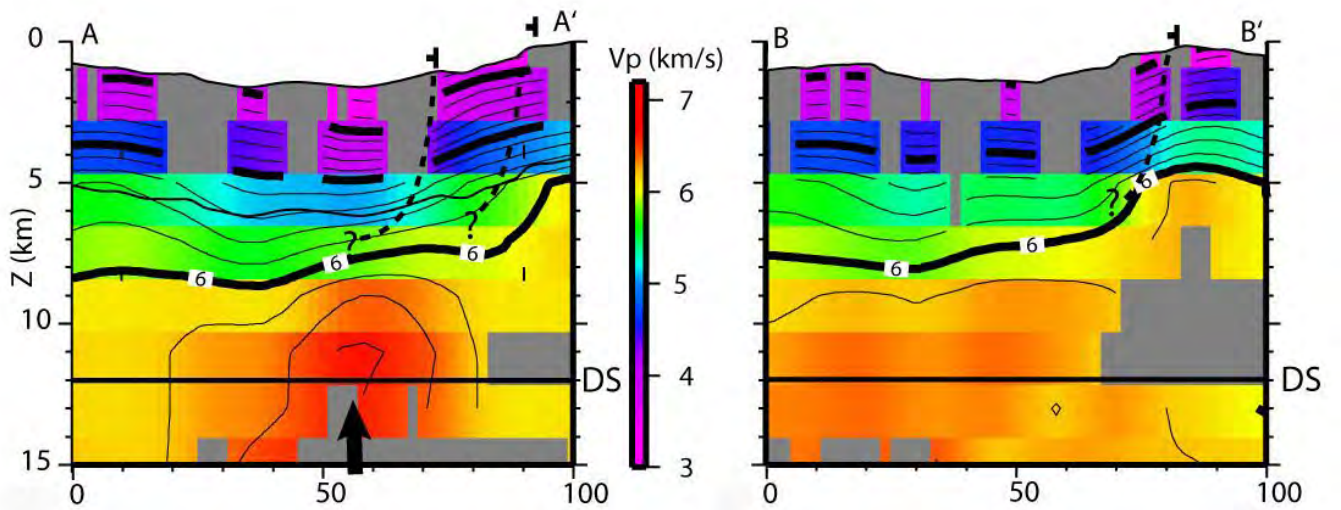
(b) Cross-sections across the NMER
