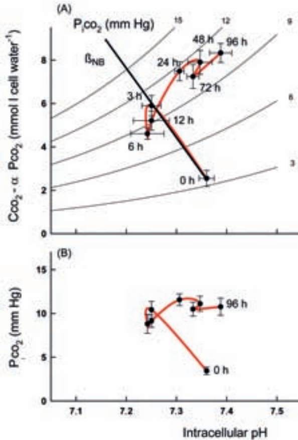
Figure 9.1 pH bicarbonate diagram (A) depicting the interrelated changes of intracellular acid-base variables pH (pH i ), bicarbonate and P CO 2 (P CO 2 ) over time and in relation to the non-bicarbonate buffer (β NB ) line. Initial changes in pH i are driven by the accumulation of CO 2 which leads to a rise in P CO 2 (B), titrates non-bicarbonate buffers and is therefore paralleled by an accumulation of bicarbonate (A). Transmembrane ion exchange and metabolic processes interfere after 3 h and, after an initial base loss, lead to continued net bicarbonate accumulation while the respiratory acidosis persists with more or less constant P i CO 2 levels (based on data from Pörtner et al. , 1998).
