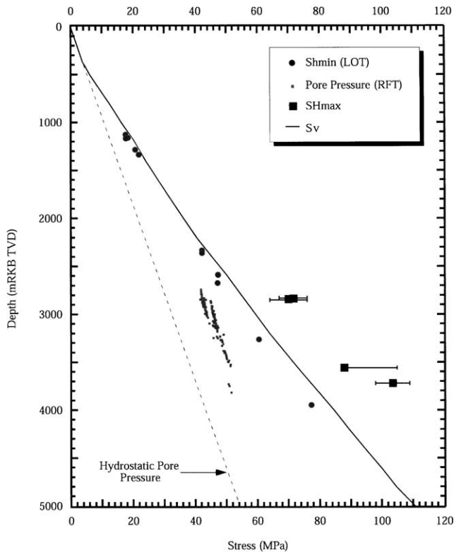
Fig. 5. Overburden stress from integration of density logs (solid block line), pore pressure measurements (small dots), S_{hmin} values determined from LOTs in different wells (larger dots) and estimates of S_{Hmax} (boxes and error bars) determined from analysis of drilling-induced tensile fractures in the Visund field of the northern North Sea (after Wiprut et al. [26]).
