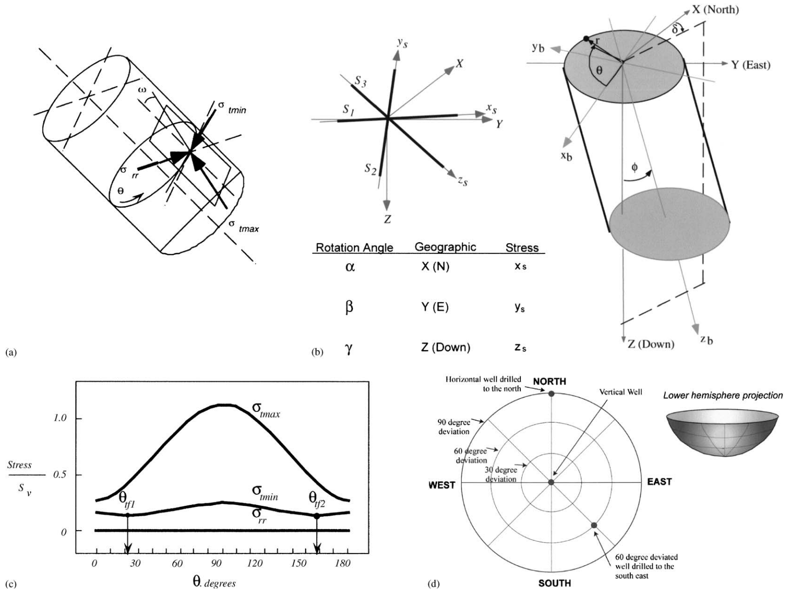
Fig. 15. (a) Stresses acting in the wall of an arbitrarily oriented wellbore, (b) coordinate system used to transform knowledge of principal stresses, to that around the wellbore, (c) variation of principal stresses around an arbitrarily oriented wellbore, and (d) lower-hemisphere projection used to display relative stability of wells with different deviations and azimuth.
