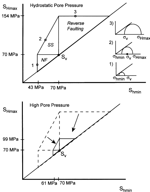
Fig. 2. Stress polygons that define possible magnitudes of S_{h\min} and S_{H\max} at any given depth as defined by Anderson's faulting theory and Coulomb faulting theory for a given coefficient of friction and pore pressure. The circumference of the polygon corresponds to a case of active faulting (see inset of upper figure). The upper figure illustrates the size of the polygon for hydrostatic pore pressure and the lower figure illustrates what happens when pore pressure is equal to 80% of the overburden. As shown in Fig. 1, there is appreciably less stress anisotropy at depth when pore pressure is high.
