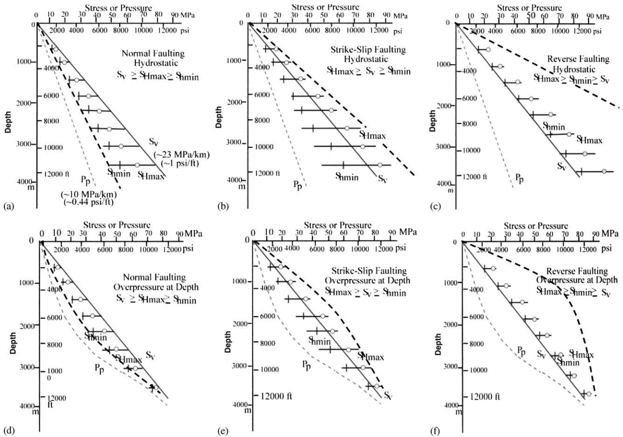
Fig. 1. Variation of stress magnitudes with depth in N, SS and RF stress regimes for hydrostatic (a–c) and overpressure conditions (d–f). Note that the difference between principal stresses increases with depth (due to the increase of crustal strength with depth but decreases as severe overpressure develops due to the decrease of crustal strength with elevated pore pressure). The heavy dashed lines indicate the limiting case for stress magnitudes based on frictional faulting theory based on Eqs. (2)–(4). Note that in cases of severe overpressure, there are very small differences between the three principal stresses, regardless of whether it is an N, SS or RF region.
