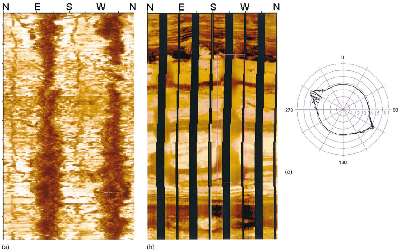
Fig. 8. (a–c) Image logs of a well with wellbore breakouts. These are manifest as dark bands (low reflection amplitudes) on opposite sides of the well in ultrasonic televiewer image logs (UBI Well A) and out-of-focus zones on electrical imaging logs (FMI Well B). By making cross sections of Well A, it is possible to clearly identify wellbore breakouts as shown on the right. Note also the existence of drilling-induced tensile fractures 90^\circ from the breakouts.
