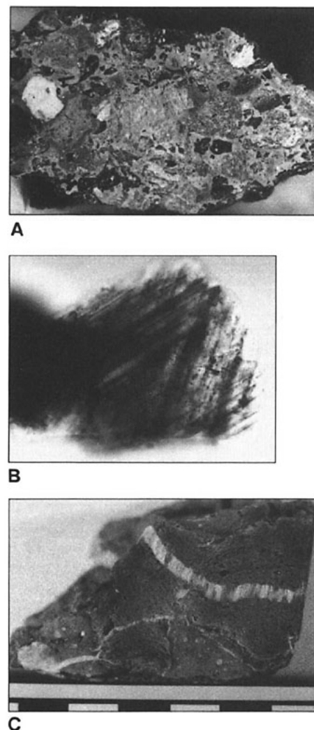
Figure 5. A: Polished slab showing polymict breccia sample Y6 N14. Specimen is 4 cm across. B: Shocked quartz grain (0.32 mm across) from polymict breccia Y6 N14. Grain shows eight sets of lamellae when rotated: two sets are visible here. C: Altered ejecta clast in polymict breccia sample Y2 N6. Note contorted internal fabric and crosscutting gypsum veins. Scale shows centimetre divisions.
