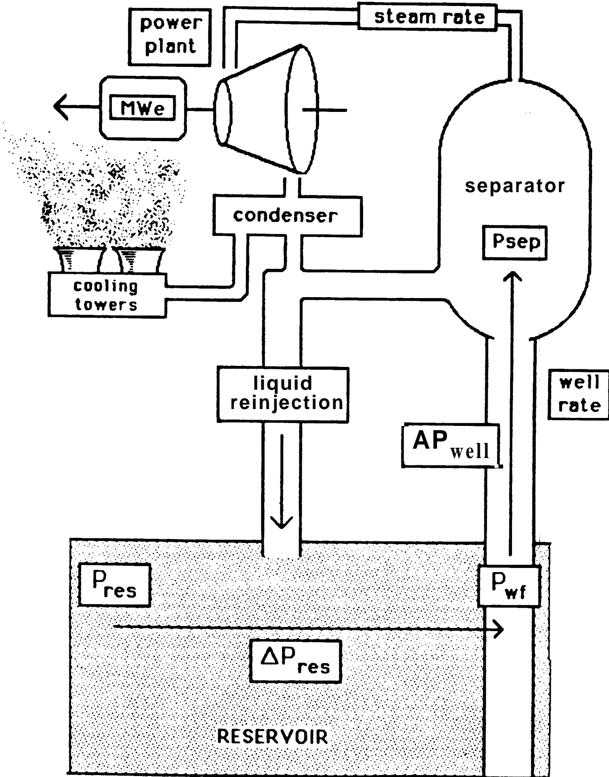
Figure 1 Physical Features of Liquid Dominated Development
