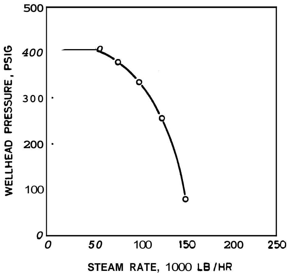
Figure 5 The Geysers • Steam Rate vs. Wellhead Pressure (Ramey 5 )
