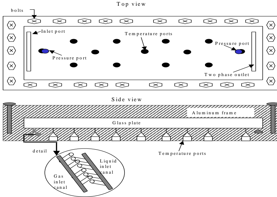
Figure 1.3: Schematic diagram of fracture apparatus.
