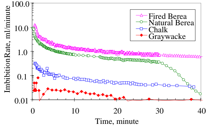
Figure 2.16: Imbibition rates in the units of ml/minute in different rocks.
