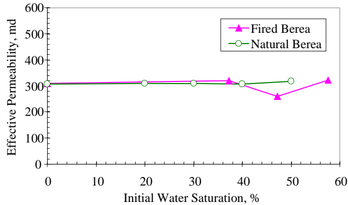
Figure 2.12: Effect of initial water saturation on effective permeability of the water phase in natural and fired Berea.
