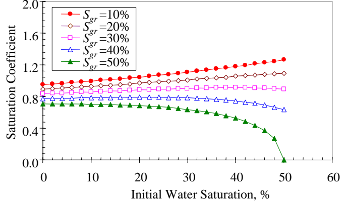
Figure 2.1: Effect of initial water saturation on saturation coefficient, which is directly proportional to recovery (GOIP) and imbibition rate (GOIP/minute).
