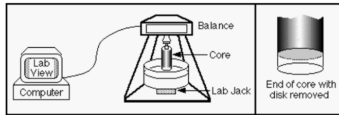
Figure 2.2: Schematic of apparatus for water imbibition test.
