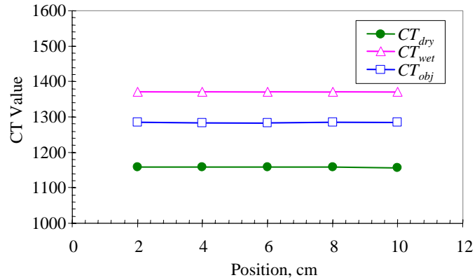
Figure 2.3: Distribution of CT values in the core when the core is dry, saturated with water, and displaced by gas.
