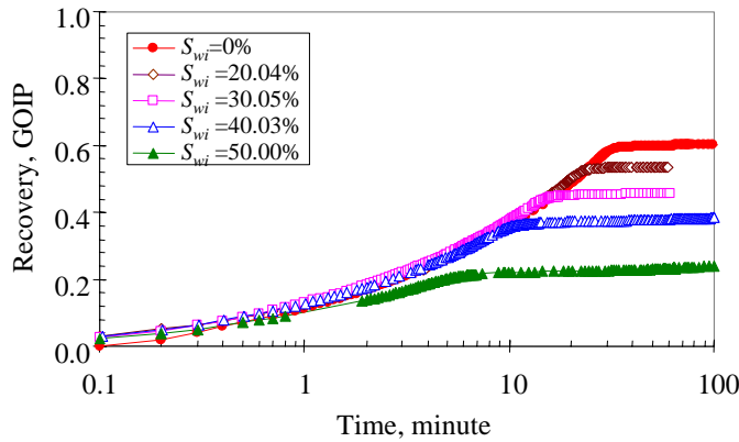
Figure 2.6: Effect of initial water saturation on gas recovery in the units of GOIP in natural Berea sandstone.
