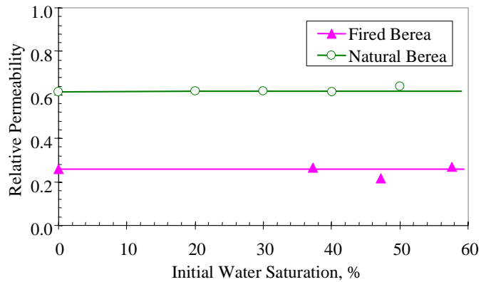
Figure 2.13: Effect of initial water saturation on relative permeability of the water phase in natural and fired Berea.
