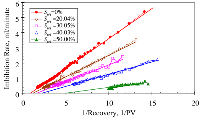
Figure 2.11: Relationship between imbibition rate and the reciprocal of gas recovery at different initial water saturations in natural Berea.
