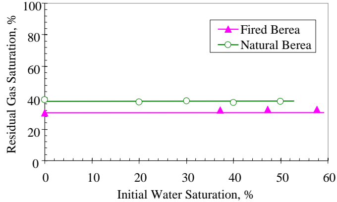
Figure 2.8: Effect of initial water saturation on residual gas saturation in natural and fired Berea.
