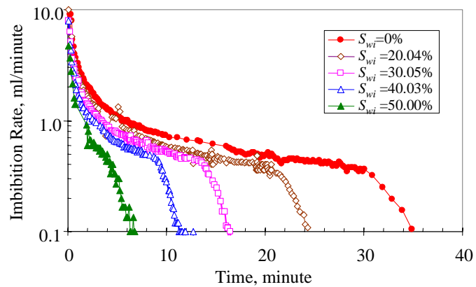
Figure 2.9: Effect of initial water saturation on imbibition rate in the units of ml/minute in natural Berea sandstone.
