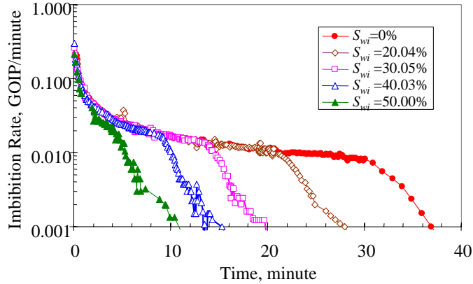
Figure 2.10: Effect of initial water saturation on imbibition rate in the units of GOIP/minute in natural Berea sandstone.
