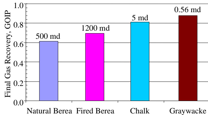
Figure 2.15: Final gas recovery (GOIP) in different rocks.
