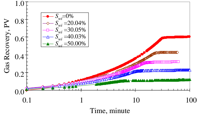
Figure 2.5: Effect of initial water saturation on gas recovery in the units of pore volume in natural Berea sandstone.
