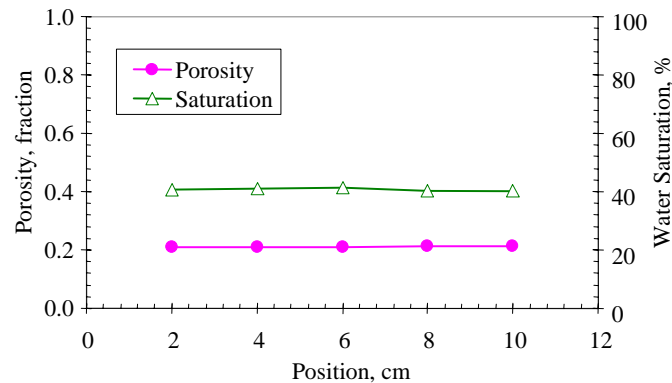
Figure 2.4: Distribution of porosity and initial water saturation in the core.
