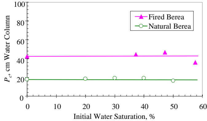
Figure 2.14: Effect of initial water saturation on capillary pressure in natural and fired Berea.
