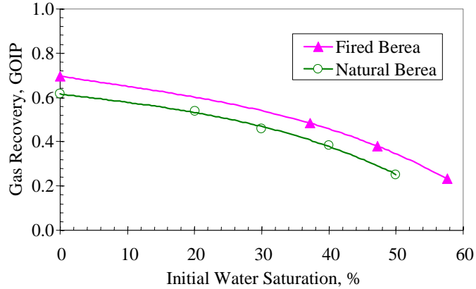
Figure 2.7: Effect of initial water saturation on final gas recovery in the units of GOIP in natural and fired Berea.
