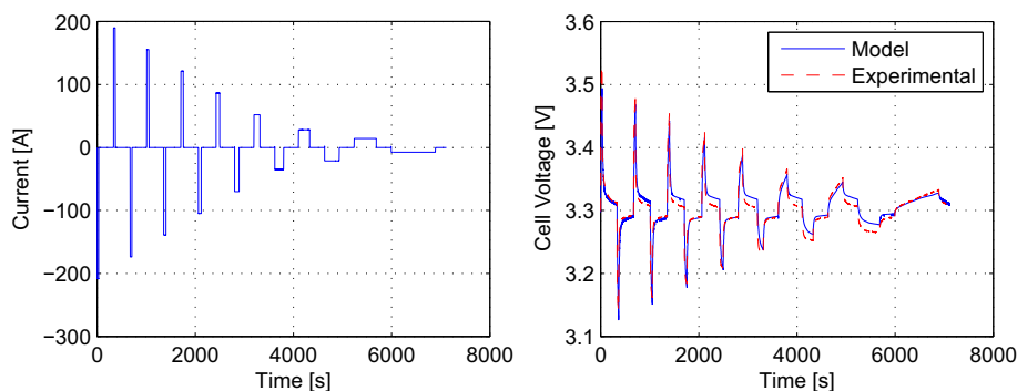
Fig. 8. Battery model validation: input current profile (left) and measured and predicted voltage (right).
