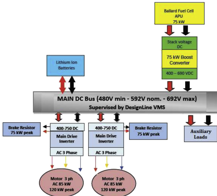
Fig. 1. Proposed bus powertrain.
