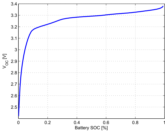
Fig. 9. V_{OC} vs. SOC curve for LFP battery cell.
