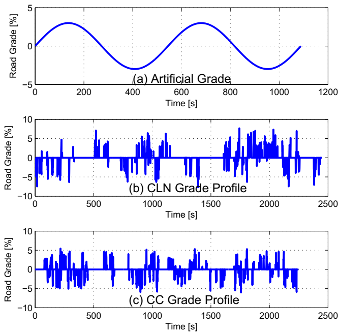
Fig. 11. Drive cycle grade profiles.
