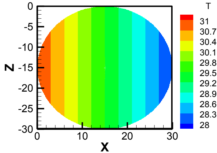
Figure 3. Initial temperature distribution used in Scenario 2. This temperature distribution is roughly estimated from kismet temperature measurements below the drift. There a large uncertainty in this assumption. The temperature difference between the injection and production well is about 1°C.
