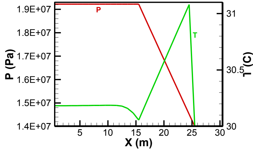
Figure 5. The temperature and pressure of the 1D column at 30 days.
