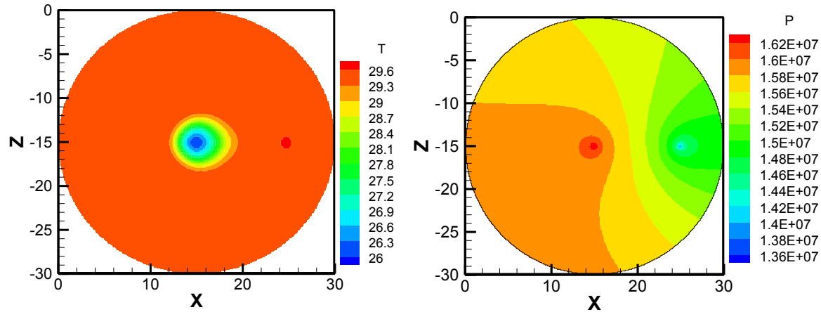
Figure 2. Temperature and pressure distribution of the fracture plane after 15 days of water injection. Note there is a slight temperature increase around the production well (0.3°C). The pressure difference between the injection-production wells is about 28bar.
