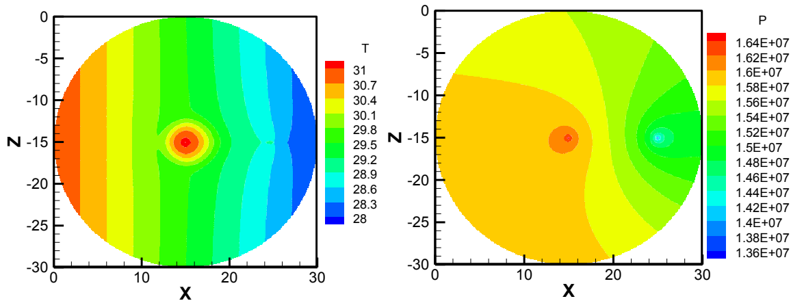
Figure 4. Temperature and pressure distribution of the fracture plane after 15 days of water injection. Again, there is a local temperature increase around the production well in addition to the temperature perturbation from the flow into the well (a total increase of 0.47°C).
