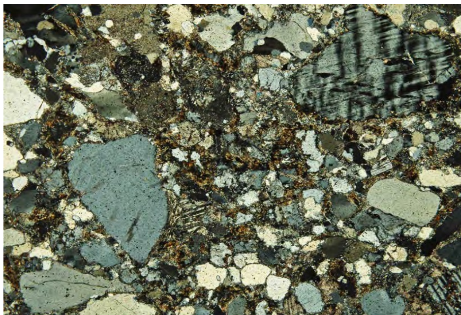
Photo 7: SAMPLE DY5ST1 (Transmitted light, crossed polarisers, Obj. x4, Image PC202562)
