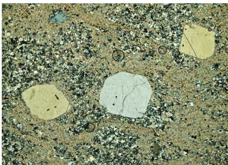
Photo 4: SAMPLE DY4ST3 (Transmitted light, crossed polarisers, Obj. x4, Image PC202574).
