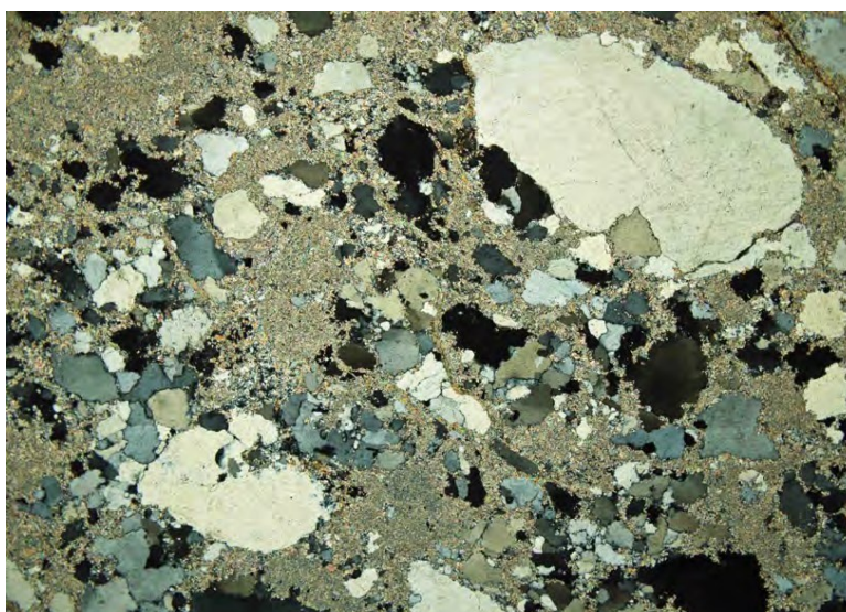
Photo 10: SAMPLE DY1ST5 (Transmitted light, crossed polarisers, Obj. x2.5, Image PC202571)
