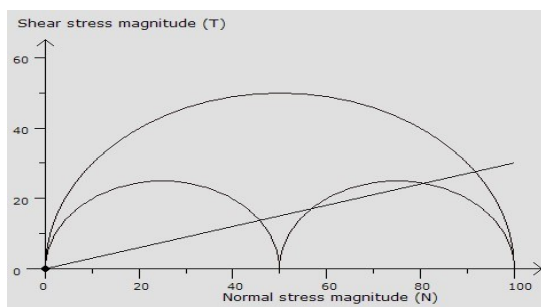
Figure 4: Structural analysis of Flow Banding
