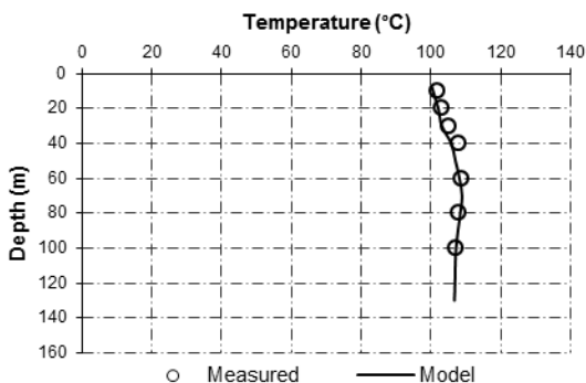
Figure 5: Temperature vs. depth profiles of the shallow B-10 well.
