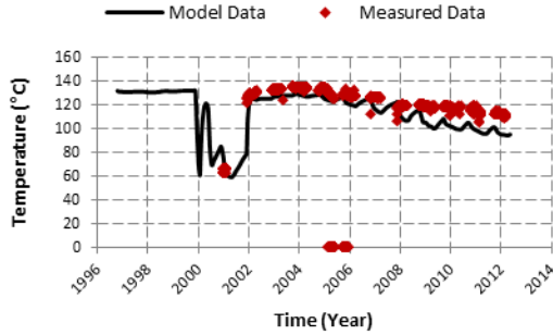
Figure 8: A comparison of simulated (model) and measured temperatures for the deep BD-2 well.
