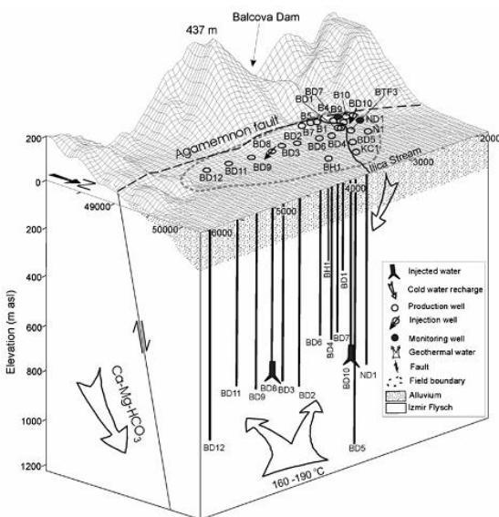
Figure 2: Conceptual model of the Balcova geothermal field (Aksoy et al., 2007).
