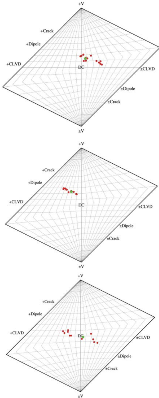
Fig. 2 Examples of confidence regions for the source types of three microearthquakes at the Coso geothermal area, California. Green symbols: best-fit solutions; red symbols: other acceptable solutions that delineate the confidence region.
