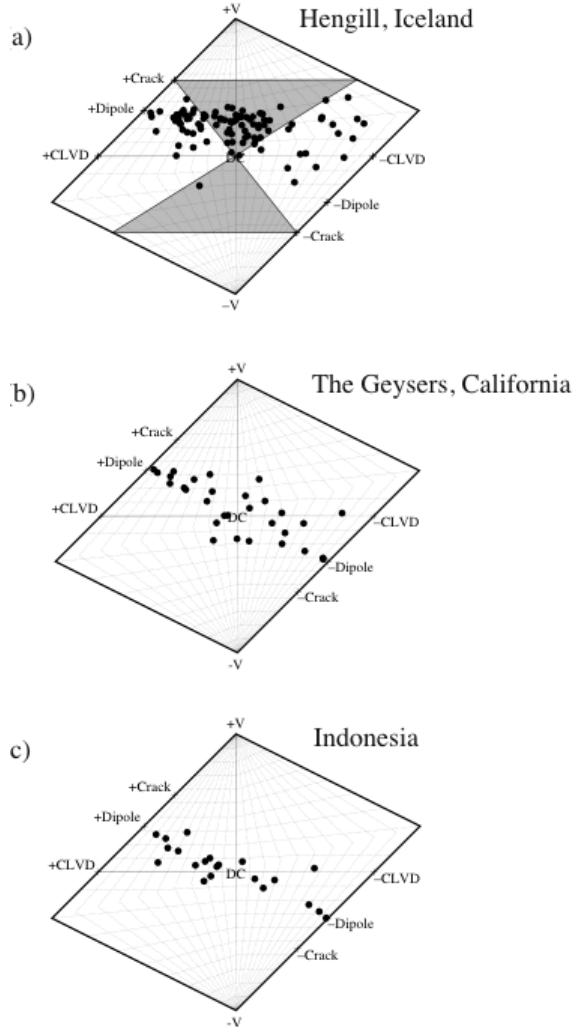
Fig. 1 Source types for microearthquakes at three geothermal areas, as determined from linear-programming inversion of seismic wave polarities and amplitude ratios. The source type depends only on the ratio of the principal moments, and is independent of source orientation.
