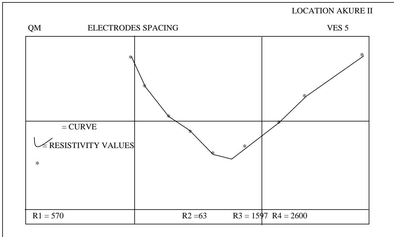
TYPICAL HA TYPE CURVE OBTAINED IN THE STATION VES 5
