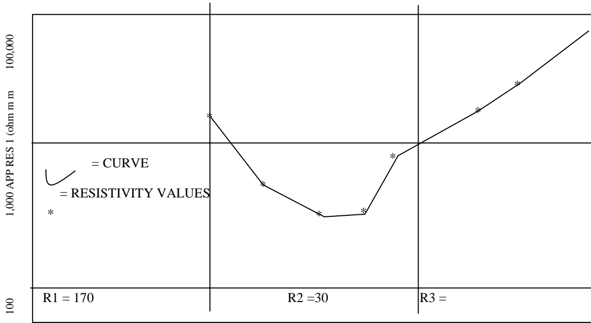
TYPICAL H TYPE CURVE OBTAINED IN THE STATION VES 4
