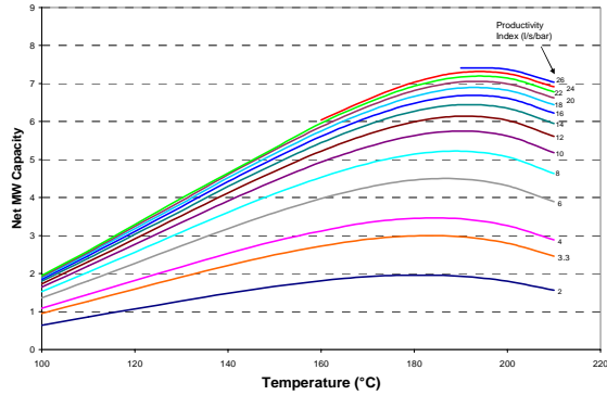
Figure 4. Net MW Capacity of a Pumped Well versus Temperature (binary-cycle power generation)
