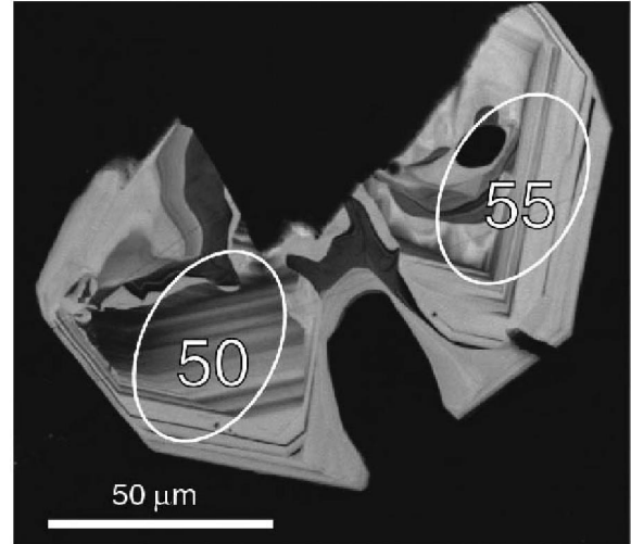
Fig. 2. Cathodoluminescence image of zircon crystal from LGM1. Dark bands correlate with areas high in U. The white circles represent areas analyzed with the SHRIMP-RG and yielded 230 Th/ 238 U ages of 50±10 and 55±10 ka (1 σ analytical errors). This crystal is among the oldest from this sample and may have been remobilized from an earlier intrusion.
