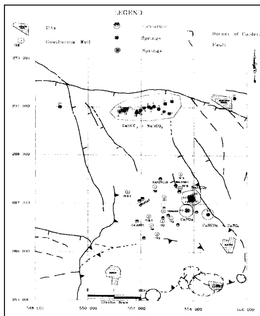
Fig.1. Location of Berlin geothermal field
