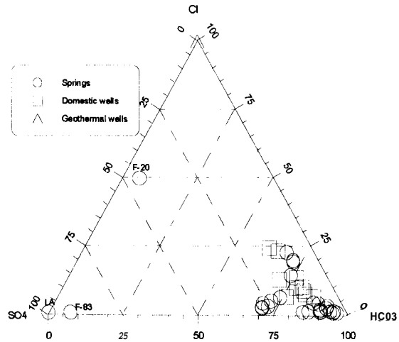
Fig. 3. Relative Cl-SO 4 -HCO 3 content in Berlin geothermal area
