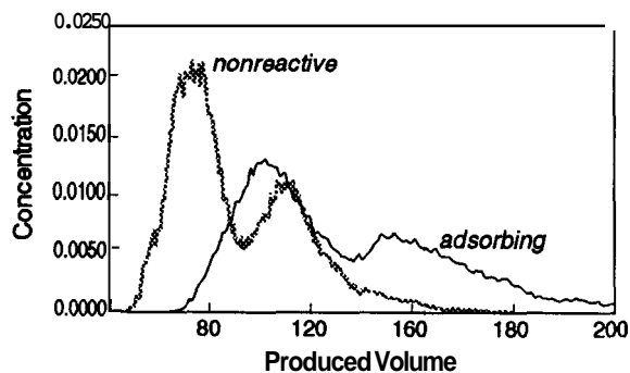
Fig. 5. A Comparison of nonreactive and adsorbing tracers at the end of a continuous reservoir circulation period of 10 years.
