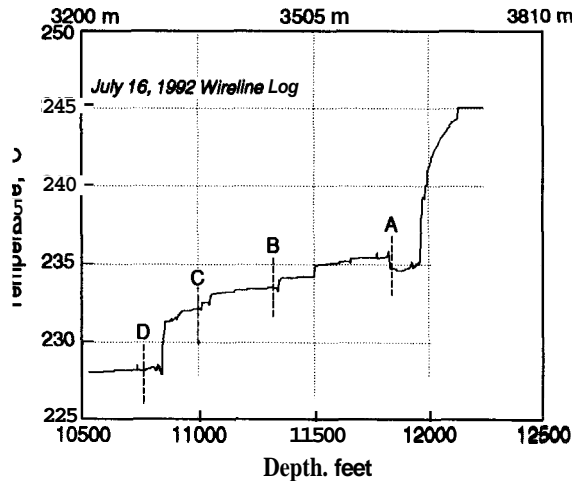
Fig. 1. A typical temperature profile across the Production Interval
