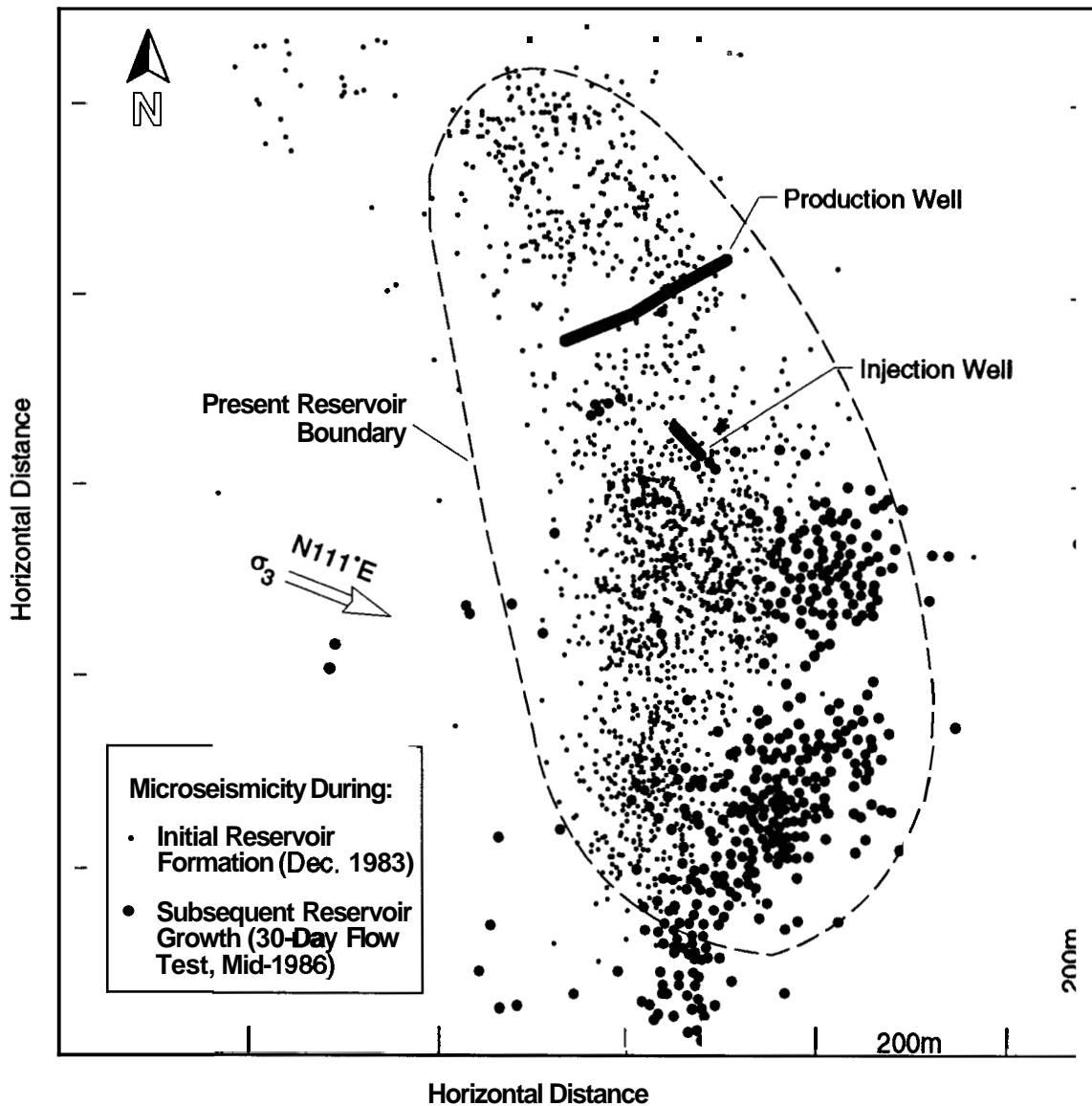
Fig. 3. Plan view of the HDR reservoir at Fenton Hill showing the microseismic event locations for the two principal episodes of reservoir growth. The large region to the south of the injection well [encompassing most of the reservoir extension that occurred during the very-high-pressure initial 30-day flow test of the reservoir in 1986 (Dash, 1989)] is essentially a stagnant part of the reservoir that is unavailable for heat transfer to the fluid flowing mostly northward from the injection well to the production well.
