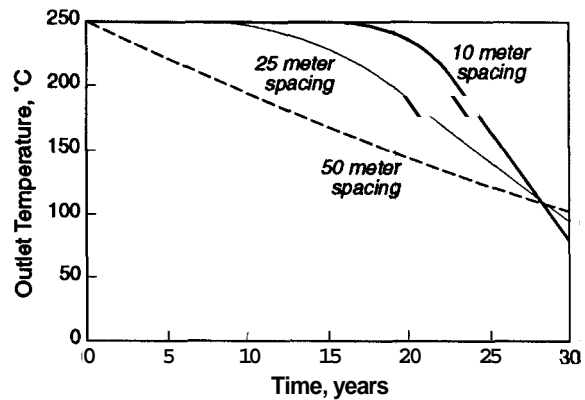
Fig. 2. The influence of joint spacing on HDR reservoir production temperature profiles for a reservoir volume of 50 million m 3 per production well, each flowing at a rate of 500 gpm (31.5 l/s). These results were obtained using the discrete element HDR reservoir simulator GEOCRACK (DuTeaux et al., 1996a, Swenson et al., 1995).
