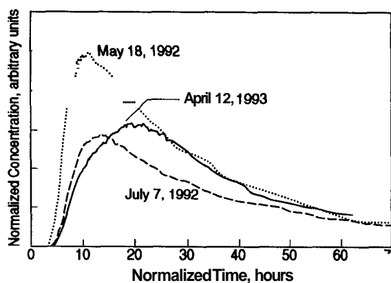
Fig. 4. Recovery of fluorescein dye tracer on three occasions; early and late during the 8-months of flow testing in 1992, and 4 weeks after renewed flow testing in 1993
