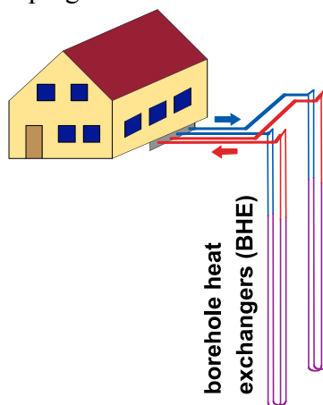
Figure 5: Basic scheme of a borehole heat exchanger installation
