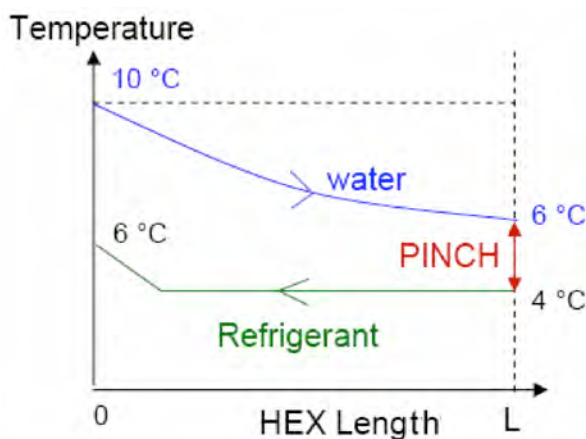
Figure 13: Temperature development in the heat pump for work package 2, over the length of the heat exchanger for evaporator (above) and condenser (below)
