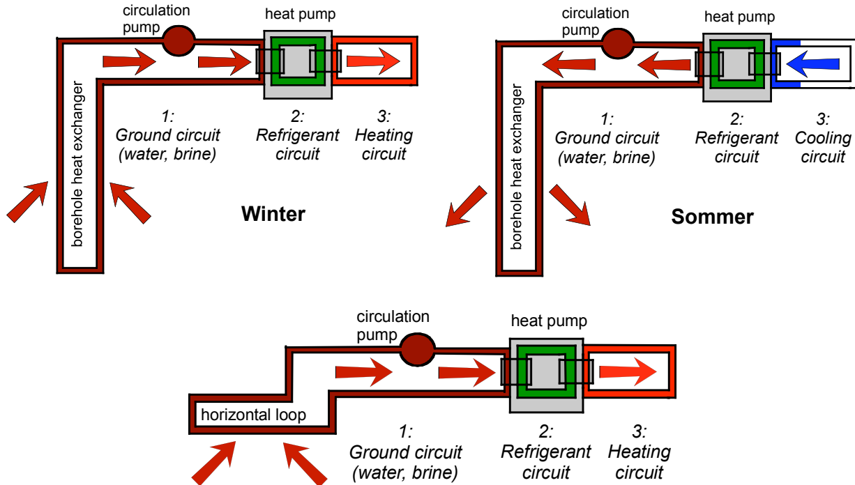
Figure 1: Basic scheme of a “classical” GSHP with water/brine circuit, with BHE or horizontal collector; this system can be reversed for cooling
