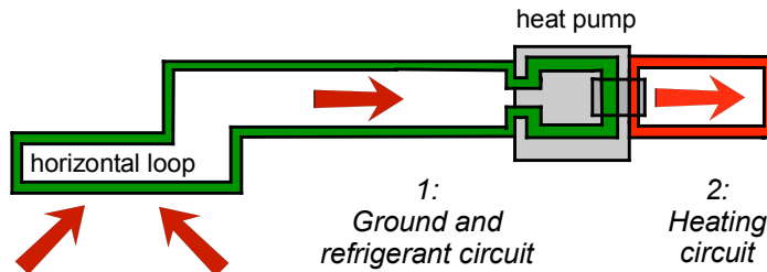
Figure 2: Basic scheme of a direct expansion GSHP with horizontal collector; this system can only be used for heating
