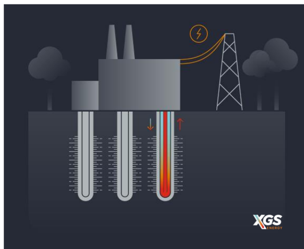
Figure 1 Example of a Closed Loop Geothermal (CLG) System (XGS Energy, 2024)
