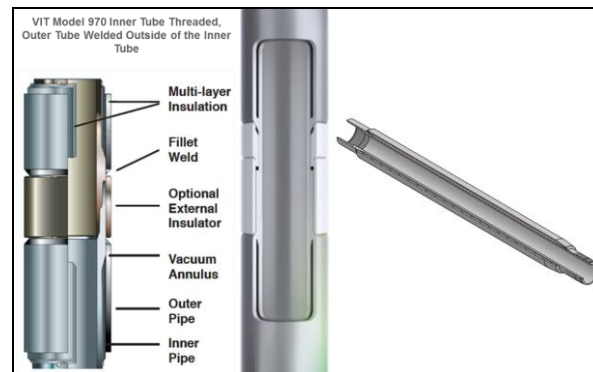
Figure 2 VIT Cross Section (Vallourec, 2024)
