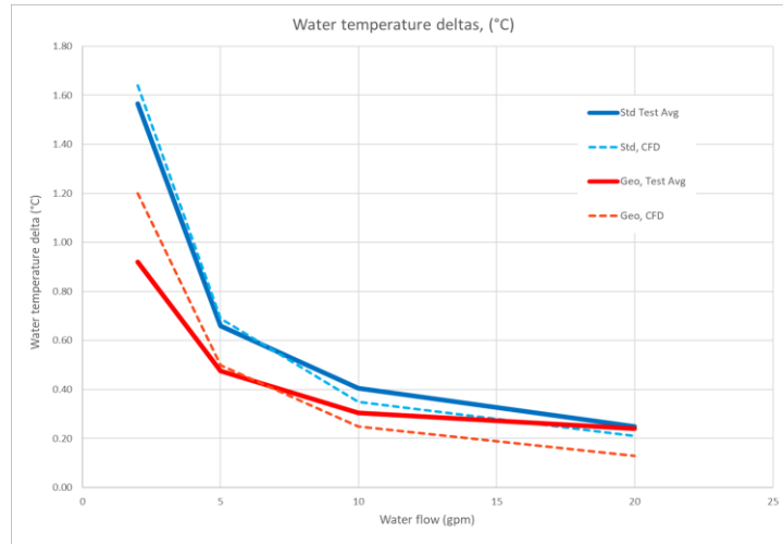
Figure 12: Comparison of physical test results to CFD simulations.
