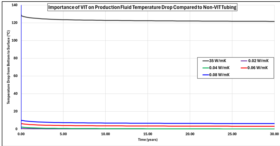
Figure 14 Importance of VIT on Production Fluid Temperature Drop Compared to Non-VIT Tubing
