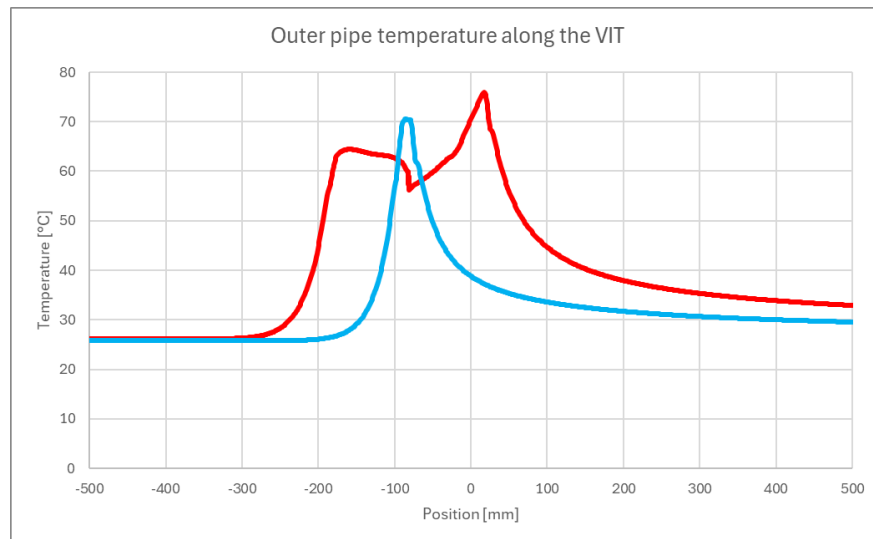
Figure 11: Temperature profile comparison between standard connection (red) and geothermal optimized connection (blue).
