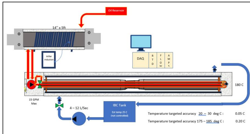
Figure 8 VIT Test Bench Setup (Dufrene et al. (2024))
