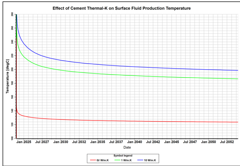
Figure 13 Effect of Cement Thermal Conductivity on Surface Fluid Production Temperature
