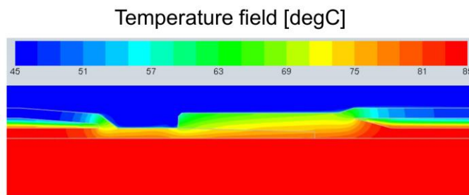
Figure 6: Temperature distribution simulation using computational fluid dynamics (CFD) analysis
