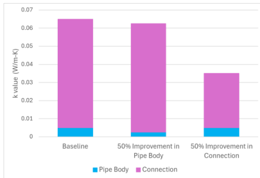
Figure 3: Combined Thermal-k comparisons of baseline case, 50% reduction of pipe body thermal-k and a 50% reduction of connection thermal-k. Adapted from Ceyhan and Vasantharajan (2021).
