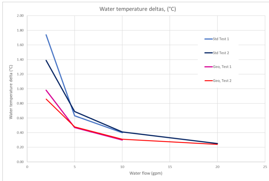
Figure 10: Comparison of lab tests of standard connection (blue) with VIT optimized connection (red).
