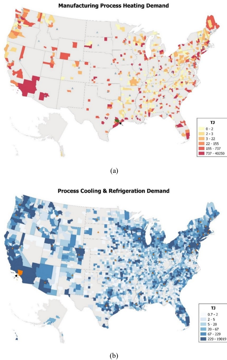
Figure 5: Manufacturing low-temperature (a) heating and (b) cooling demand by U.S. county. The county where heating and cooling demand is highest is highlighted with green or orange background and black arrow.
