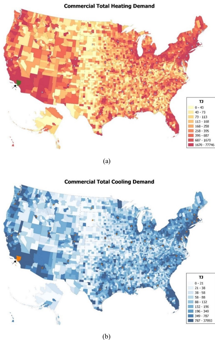
Figure 4: Commercial (a) heating and (b) cooling demand by U.S. county. The county where heating and cooling demand is highest is highlighted with green or orange background and black arrow.
