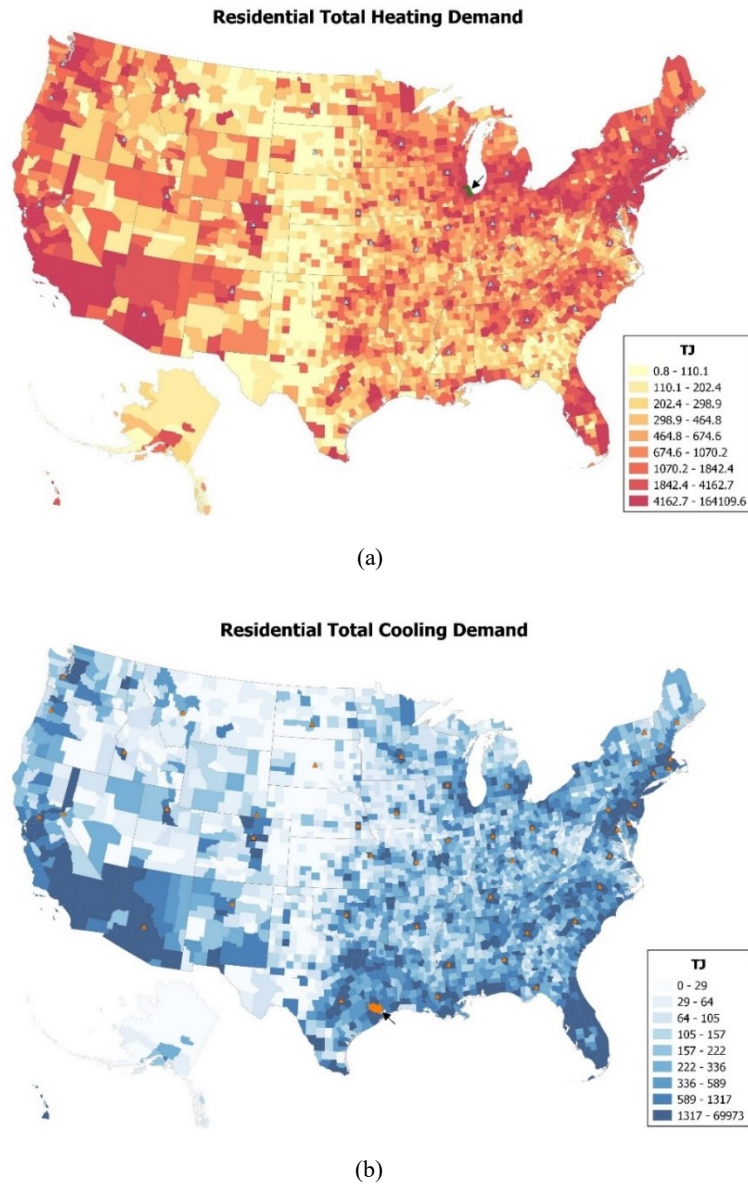
Figure 3: Residential (a) heating and (b) cooling demand by U.S. county. The county where heating and cooling demand is highest is highlighted with green or orange background and black arrow.
