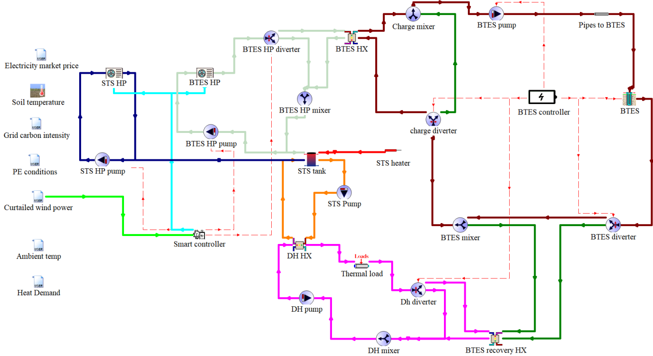
Figure 3: Simplified schematic of the TRNSYS model of the proposed energy system for King’s Buildings. For clarity, only the main connections between different modules are shown and auxiliary components are omitted. “HP” stands for heat pump, “HX” for heat exchanger, “STS” for short-term store, and “DH” for district heating.
