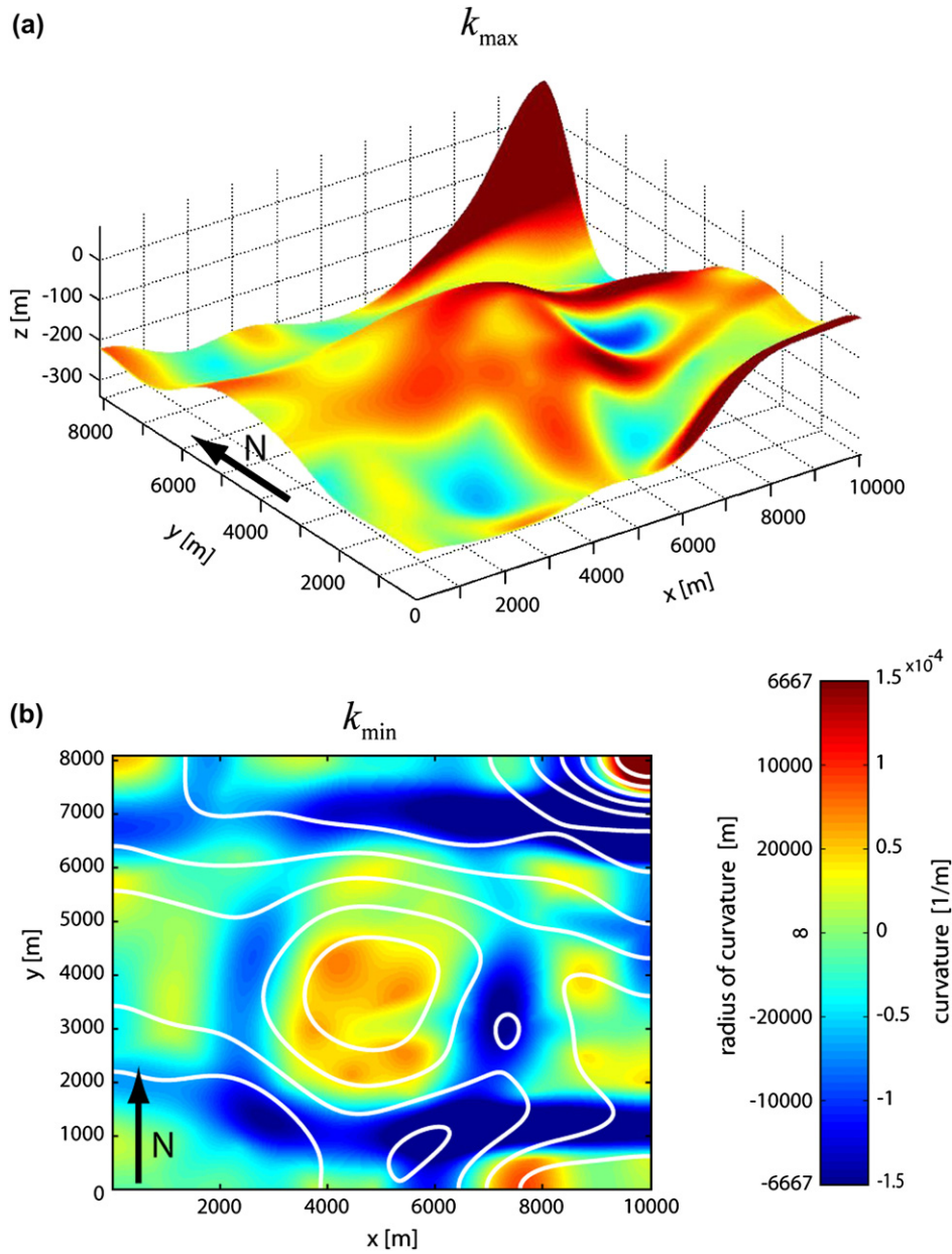
Fig. 6. Principal curvature magnitudes for 3-D depth migrated, seismically mapped horizon from the North Sea. (a) Maximum principal curvature, k_{\max} mapped onto oblique 3-D view of the horizon. (b) Minimum principal curvature, k_{\min} . White lines are elevation contours.
