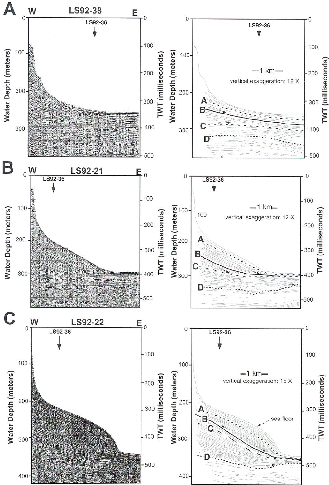
FIG. 17.—Interpreted high-resolution, single-channel, dip-oriented seismic profiles (location of lines in Fig. 8; energy source was an SSI [Seismic System Inc.] 15-in. 3 water gun), showing the variable thickness of sediment along the slope of the western margin of the Turneffe Basin. The seismic lines are displayed from north (A) to south (C). Reflectors A to D have been identified and used for correlation in the seismic lines throughout the Turneffe Basin (see Figs. 12, 14, 16). (A) Dip-oriented seismic line north of the lowstand shelf-edge delta. The wedgelike slope deposit is very thin. (B) Dip-oriented seismic line between the lowstand shelf-edge delta and the slope fan. The slope sedimentary wedge displays a slight bulge. Reflectors B, C, and D identified in this wedge of slope sediment correlate with reflectors B, C, and D identified in the progradations that are observed beneath the barrier and back-barrier reef in the multichannel line (Fig. 12). (C) Dip-oriented seismic line across the lowstand slope fan. Note the slight bulge, mainly formed by reflectors that do not appear to connect with the barrier reef to the west. These reflectors are thought to represent an accumulation of reworked deltaic sediment by southward-flowing longshore currents transported from the lowstand shelf-edge delta. TWT = two-way travelttime.
