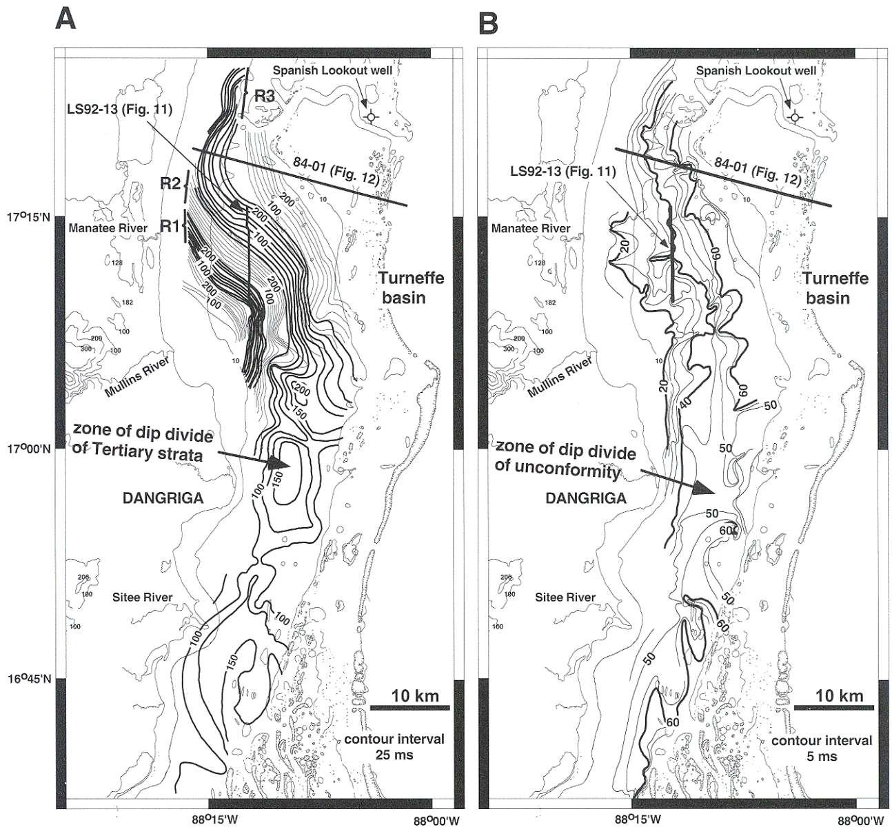
FIG. 13.—(A) Contour map of three upper Tertiary seismic horizons R1, R2, and R3 identified below the sea floor of the Southern Shelf Lagoon (Fig. 11). The R3 horizon displays a high, plateaulike area offshore Dangriga where the lowstand drainage system of valleys incised during the last glacial maximum shows a clear divide (see Figs. 8, 9). In the area north of the elevated plateau, the R1, R2, and R3 horizons dip toward the northeast, whereas in the area south of the plateau, the R3 horizon dips toward the south. (B) Contour map of the Belize unconformity identified below the sea floor of the Southern Shelf Lagoon (Figs. 5, 6, 11). The Belize unconformity displays a high, plateaulike elevated area offshore Dangriga where the lowstand drainage system of valleys incised during the last glacial maximum shows a clear divide (see Figs. 8, 9).
