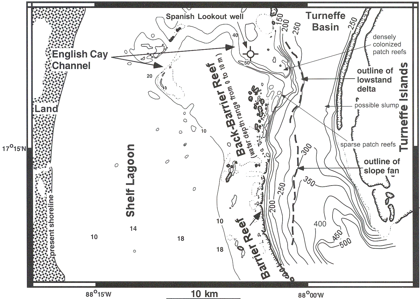
FIG. 4.—Detailed bathymetry of Turneffe Basin, the English Cay Channel, and the northern part of the Southern Shelf Lagoon at the western entrance of the English Cay Channel. Contour intervals are 10 m in Turneffe Basin and the English Cay Channel and 1 m in the Southern Shelf Lagoon. The overall southward-sloping floor of the Southern Shelf Lagoon is shown in Figure 3. From its entrance to its mouth, the English Cay Channel exhibits an eastward-sloping bathymetry. This map also shows a lowstand shelf-edge delta and a lowstand slope fan. Note also that the shallowest part of the Turneffe Basin sea floor is located in front (i.e., east) of the mouth of the English Cay Channel.
