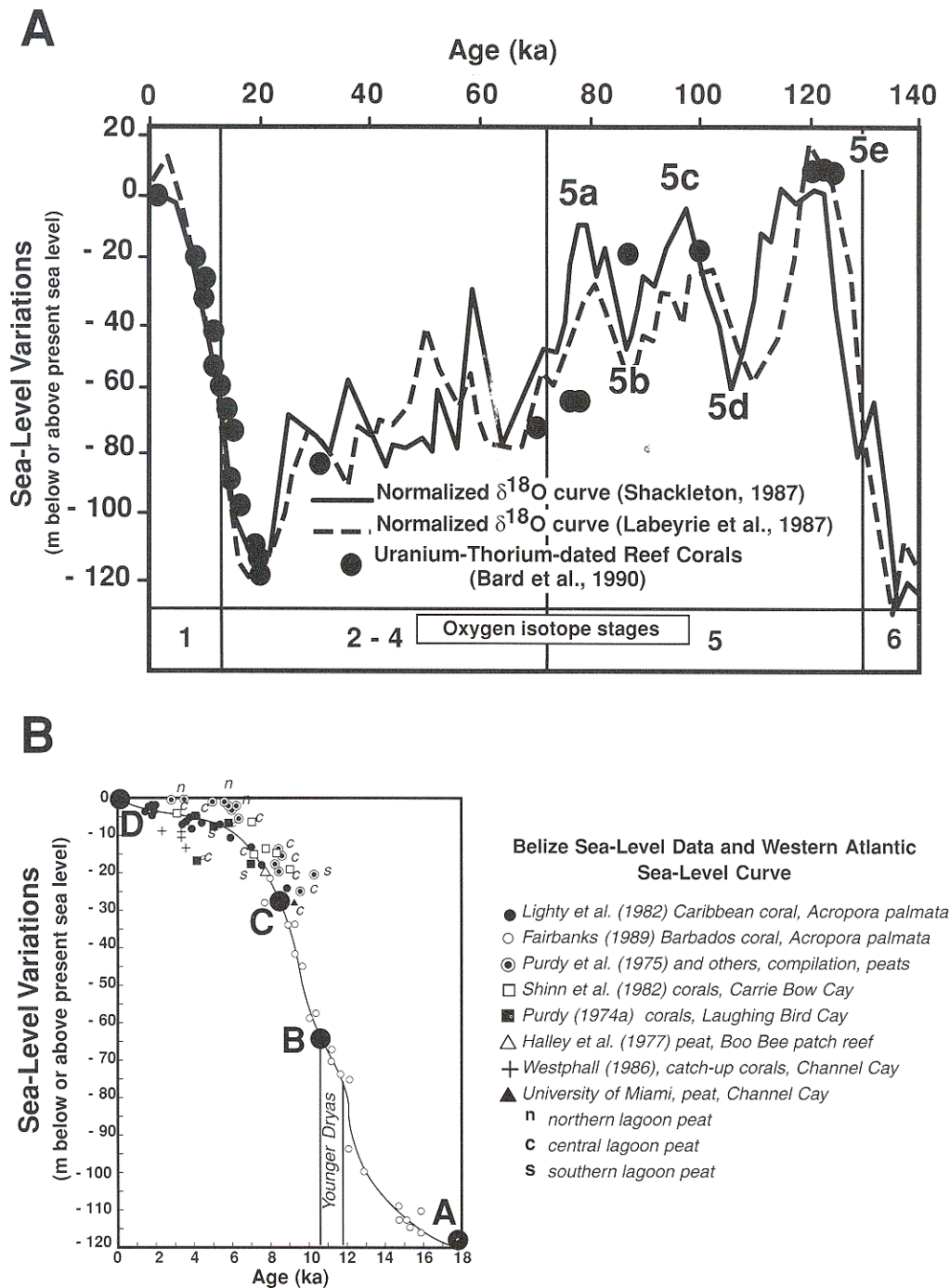
FIG. 1.—Sea-level variations for (A) the past 140 k.y. based on oxygen isotope data and dating of coral and peat samples by ^{14}\text{C} and U-Th methods and (B) the past 18 k.y. Letters A to D indicate the estimated levels of the ocean during four time intervals described in the model shown in Figure 18, which describes the evolution of the mixed siliciclastic-carbonate Belize system during the last sea-level cycle.
