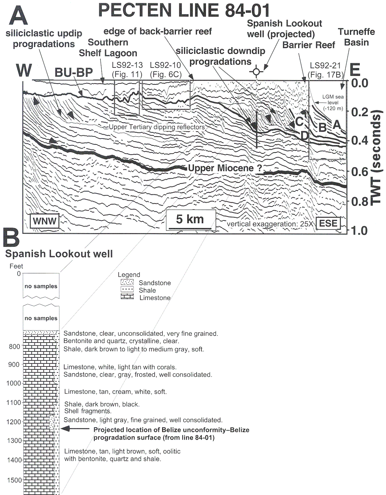
FIG. 12.—(A) Interpretation of multichannel seismic line 84-01 (located in Figs. 8, 13) and its correlation with the projected Spanish Lookout well. The outlined boxes indicate the projection of the high-resolution seismic lines shown in Figures 6C, 11, and 17B. The Belize unconformity truncates the top of the siliciclastic up/dip progradation complex in the west part of the seismic line and becomes a downlap surface for the siliciclastic down/dip progradation complex observed beneath the barrier and back-barrier reef system in the east part of the seismic line. These progradations appear to be connected to wedges of sediment (LS92-21, Fig. 17B) associated with the lowstand shelf-edge delta and slope fan (LS92-39, Fig. 14A; LS92-22, Fig. 17C). Reflectors A to D can be correlated from this multichannel line to the high-resolution lines in Turneffe Basin (see Figs. 14A, 16A, 17B). The modern reef overlies wedges of down/dip progradations. In Figure 12B, a schematic representation of the lithology at the Spanish Lookout well shows intercalations of siliciclastic and carbonate sediment in the interval corresponding to the down/dip progradations. TWT = two-way traveltime.
