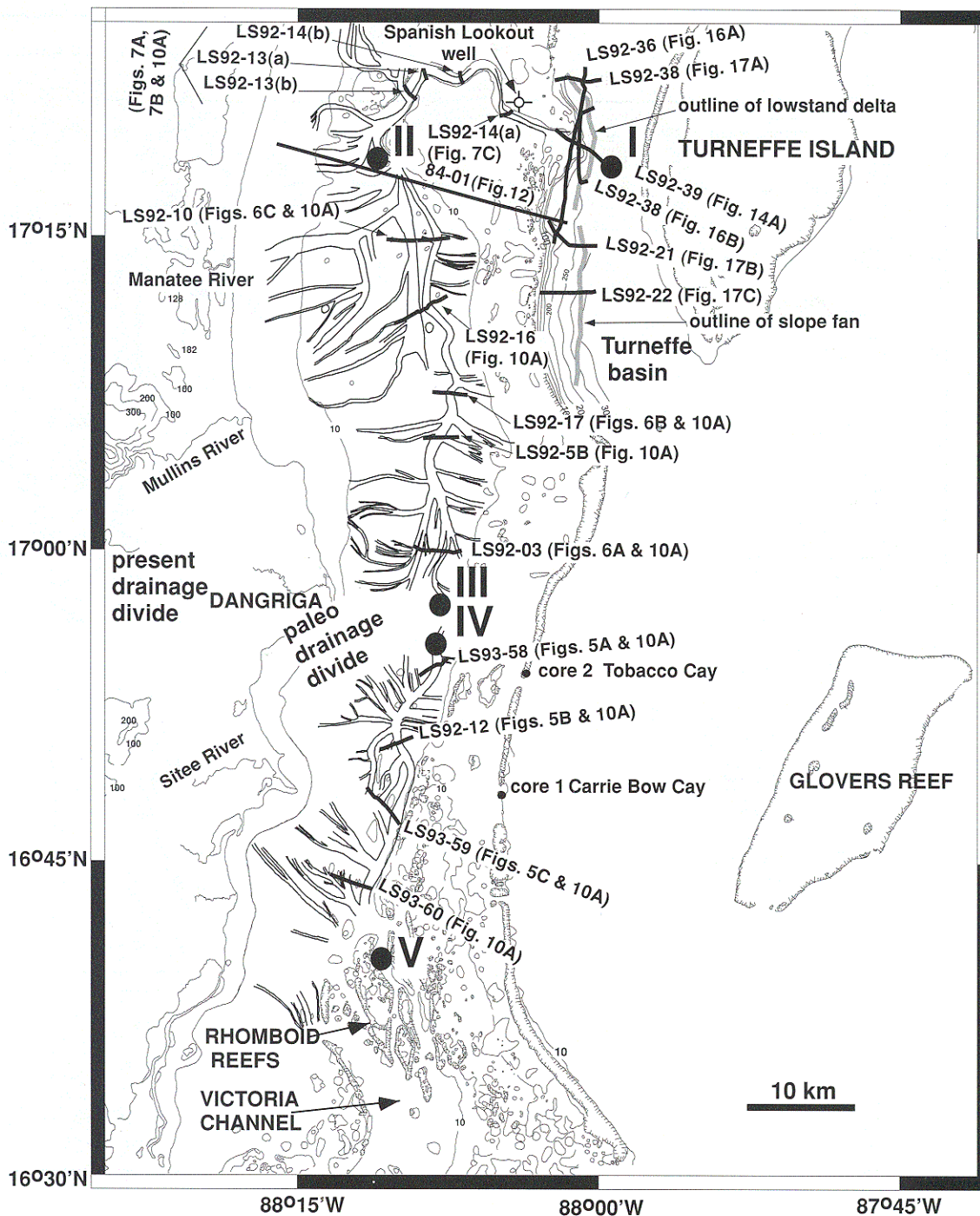
FIG. 8.—Paleodrainage during the last glacial maximum, 18–20 ka. Locations I to V are the positions of stations along the maximum incision of the main valley systems. Successive values of maximum incision were used to calculate the valley systems' gradient along the segment south of Dangriga (IV to V), the segment north of Dangriga (III to II), and the segment of English Cay Channel (II to I), shown in Figure 10B. Note how the complex drainage system north of Dangriga merges into the English Cay Channel and that the system south of Dangriga drains into the modern Victoria Channel complex. Compare the position of the paleo-drainage divide offshore Dangriga with the position of the dip divides of the upper Tertiary strata and the Belize unconformity (see Fig. 13).
