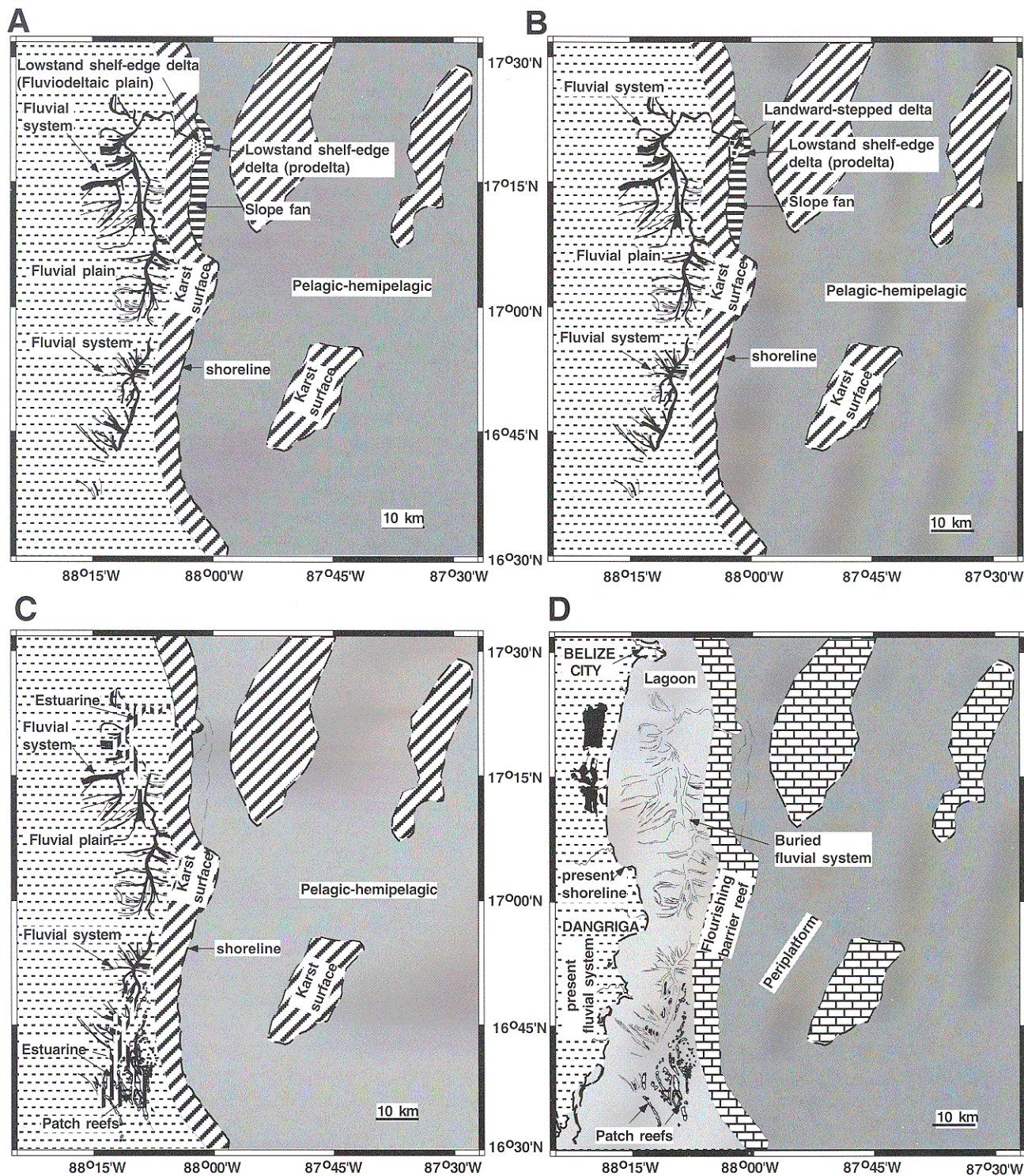
FIG. 18.—Model for the evolution of the mixed siliciclastic-carbonate system along the Belize margin during the last sea-level cycle. Letters A to D in Figure 1B indicate the estimated sea level at each of four time intervals described in the model. (A) During the last glacial maximum, 18–20 ka, the lowstand shoreline was located in front of (i.e., east of) the position of the modern barrier reef. A complex drainage system of incised valleys was developed in the lowstand fluvial plain parallel to and west of the exposed oxygen isotope stage 5 barrier reef. The drainage system south of Dangriga merged into the modern rhomboid reefs, whereas the drainage system north of Dangriga merged into a single incised valley of the English Cay Channel. A lowstand shelf-edge delta and associated slope fan were deposited at the mouth of the English Cay Channel along the western margin of the Turneffe Basin, located where the coastline was during the lowstand. (B) During the Younger Dryas, 11.8–10.6 ka, the rates of sea-level rise decreased, and sea level may have remained constant for about 1 k.y. As a result, a landward-stepped delta formed on top of the lowstand shelf-edge delta. (C) About 8.5 ka, the sea started to transgress across some parts of the lowstand fluvial plain, today the Southern Shelf Lagoon. Estuaries formed in the areas north and south of Dangriga. In the north, the estuaries were still funneled through the English Cay Channel. These environments therefore remained restricted. In the south, however, the estuaries were directly connected to the open sea, which probably favored the growth of patch reefs on river levees. Note that the dominant depositional environment in the shelf area was still siliciclastic. (D) During the past 7 ka, the sea flooded the top of the karst-modified barrier reef to establish the mixed siliciclastic-carbonate system that exists today.
