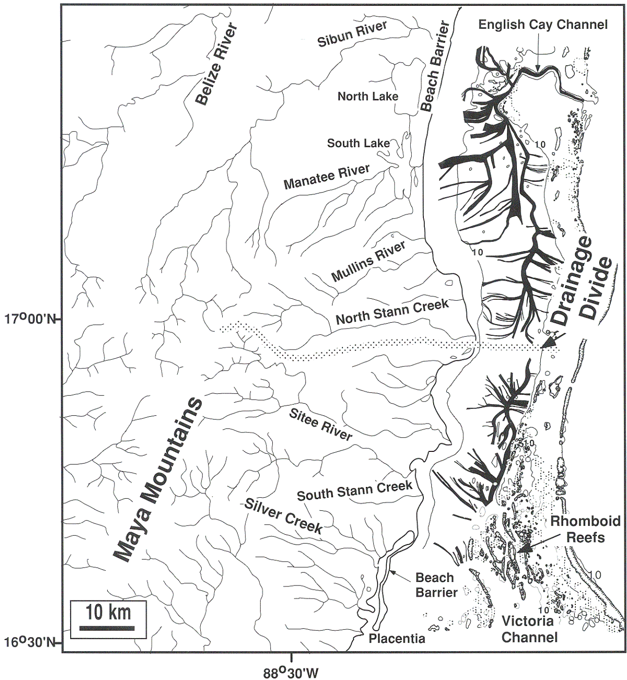
FIG. 9.—Comparison of the present onshore drainage with the paleodrainage during the last glacial maximum. The divides for both drainage systems at about lat 17°N appear to be connected.
