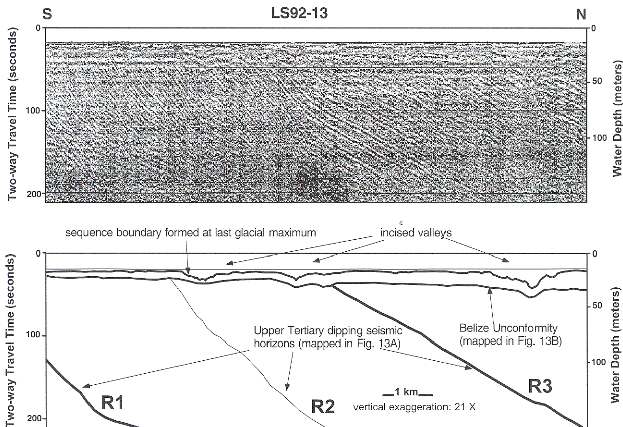
FIG. 11.—Segment of a south-to-north high-resolution single-channel seismic line located in the Southern Shelf Lagoon between Dangriga and the western entrance of the English Cay Channel located in Figure 13. Interpretation of the seismic line segment is shown in accompanying line drawing. Also shown are details of the relationship between the upper Tertiary dipping seismic reflectors, the Belize unconformity, and the incised valleys. The upper Tertiary seismic horizons R1, R2, and R3 as well as the surface representing the Belize unconformity are mapped in Figure 13.
