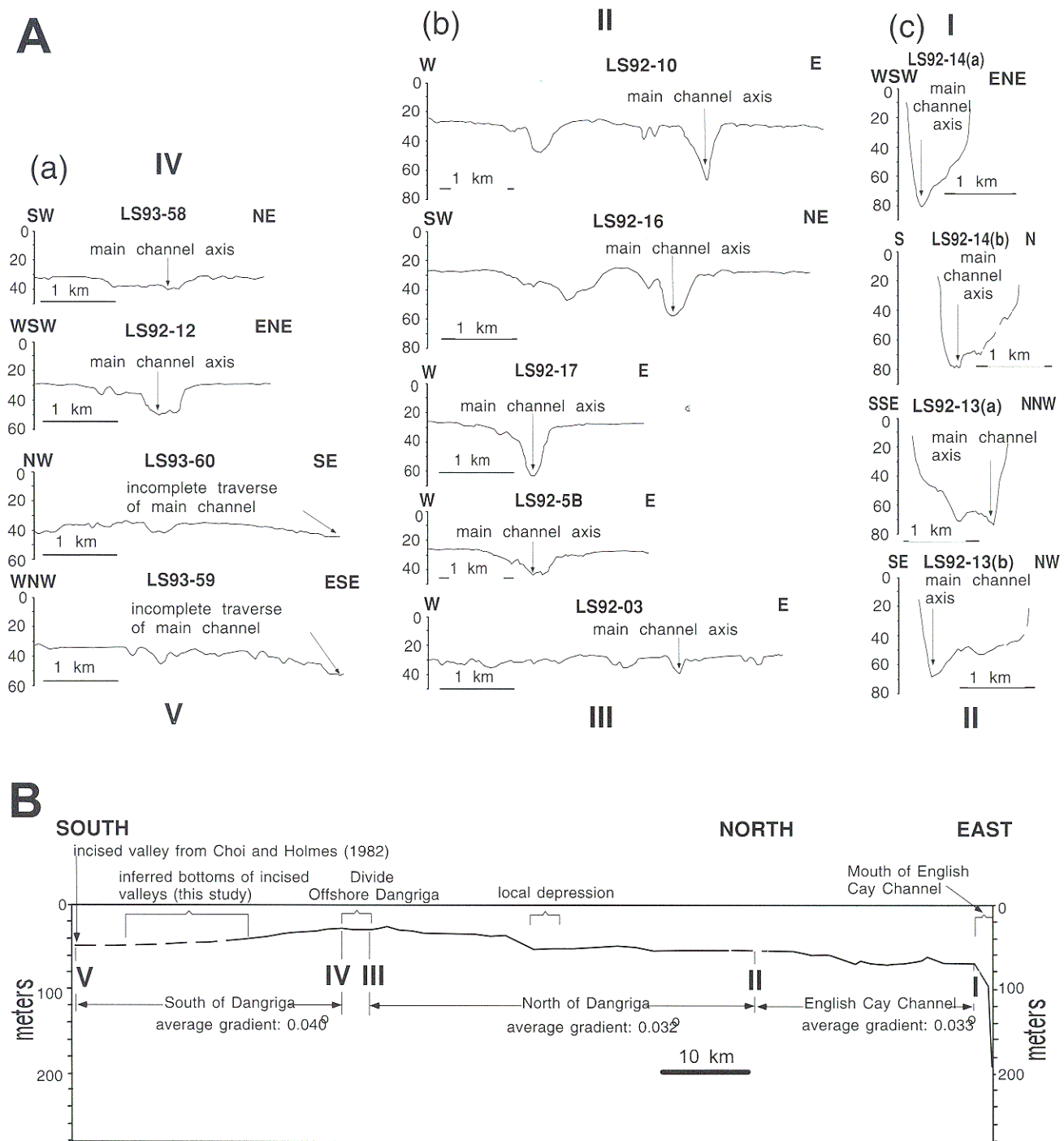
FIG. 10.—Cross sections of the valleys incised in the northern part of the Southern Shelf Lagoon and the English Cay Channel during the LGM, based on high-resolution seismic lines and the overall estimated sea-floor gradients. (A) Cross sections of incised valleys in three segments of the paleo-drainage system (located in Figs. 8, 9). (a) South of Dangriga, segment from IV to V. (b) North of Dangriga, segment from II to III. (c) English Cay Channel, segment from I to II. Vertical scale is two-way traveltime in milliseconds. (B) The longitudinal profiles of the main LGM incision, north and south of Dangriga, and along the English Cay Channel.
