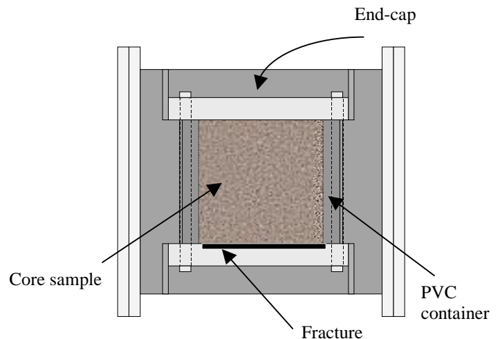
Figure. 2. The Core Holder. Lateral View.
