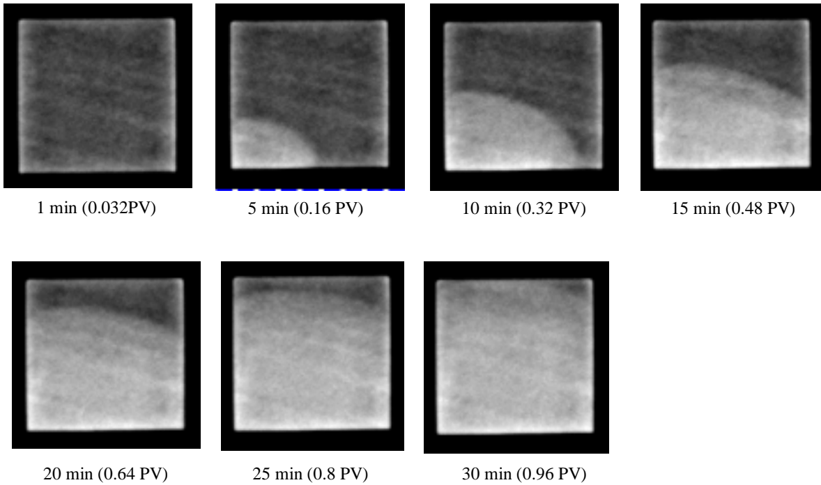
Figure. 9. CT Images for ‘Filling-fracture’ system for different times. Water injection at 1 cc/min in a fracture 0.1 mm thick.
