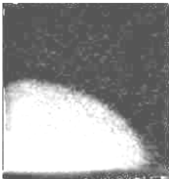
Figure. 5. CT Saturation Image for 0.32 PV injected. "Filling-fracture." Aperture = 0.1 mm.
