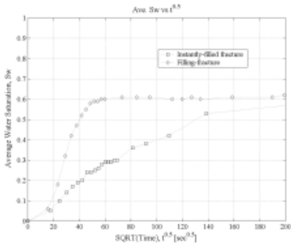
Figure 7. Average saturation versus square root of time.
