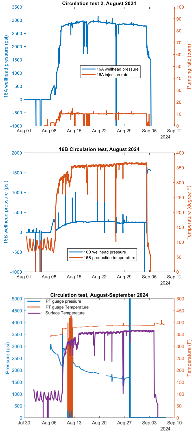
Figure 2: Data for the one-month circulation test in August-September 2024, including injection rate, injection pressure, production wellhead pressure, the production temperature, and downhole PT gauge data.
