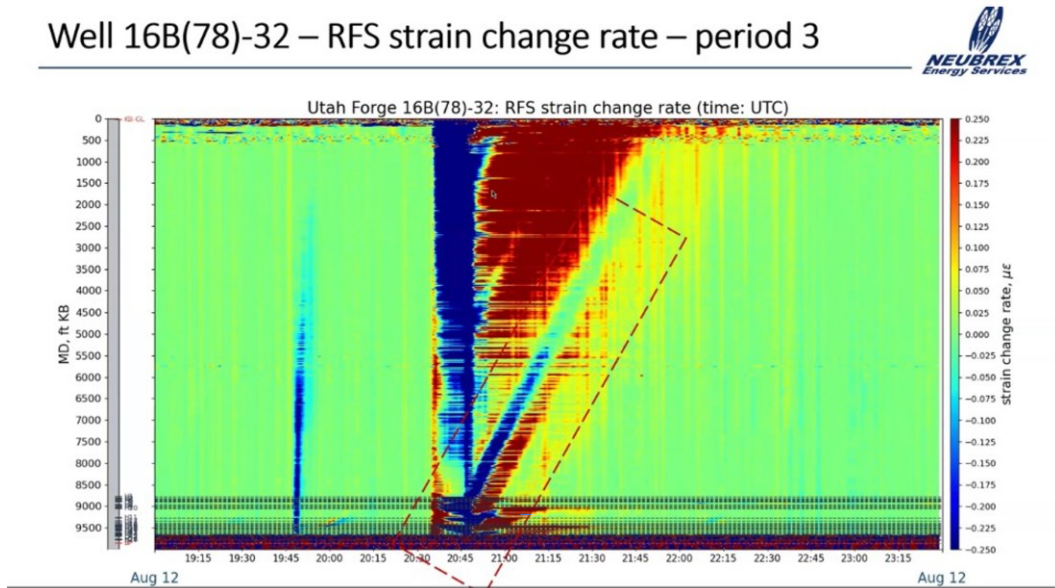
Figure 6: Fiber optic sensing strain data on August 12, 2024, during the circulation test (adapted from Jurick et al., 2024).
