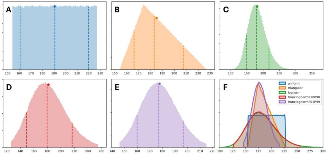
Figure 2: A.-E. Histograms generated from random-sampling distributions of the Silver Peak reservoir temperature values (low, mid, high = 154°C, 174°C, 227°C) 1 million times and visualizing with 100 bins. Plots are normalized such that the total area in each histogram equals 1. Vertical dashed lines indicate the P10, P50, and P90 locations in the distribution. The circle marker illustrates the mean. Distribution choices include A. uniform, B. triangular, C. lognormal, D. lognormal with low and high inputs treated as P10 and P90 locations, then truncated at P01 and P99, E. lognormal with low and high inputs treated as P01 and P99 locations, then truncated at P01 and P99. F. Overlay of KDE representations of the sample distributions to show relative proportions and breadth.
