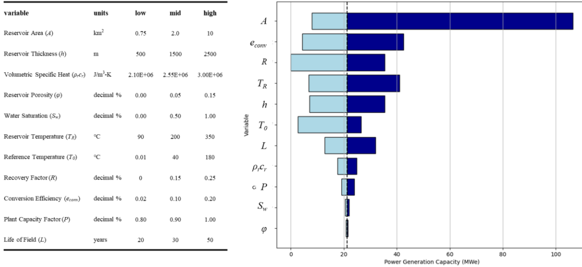
Figure 3: Sensitivity testing of the USGS method. The vertical dashed line shows results when middle values are used for each variable, while horizontal bars show the range of outcomes as the respective variable’s low/high values are applied. Variables are sorted to show the most influential at the top. Each input variable’s range was based on resource estimation literature or real-world examples. For visualization purposes, the high-side area is restricted to 10 km 2 , even though some fields exceed this size.
