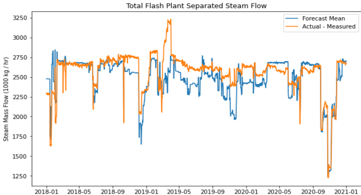
Figure 6: Flash plant historical vs. hindcast results showing a good match for stable periods of operation.
