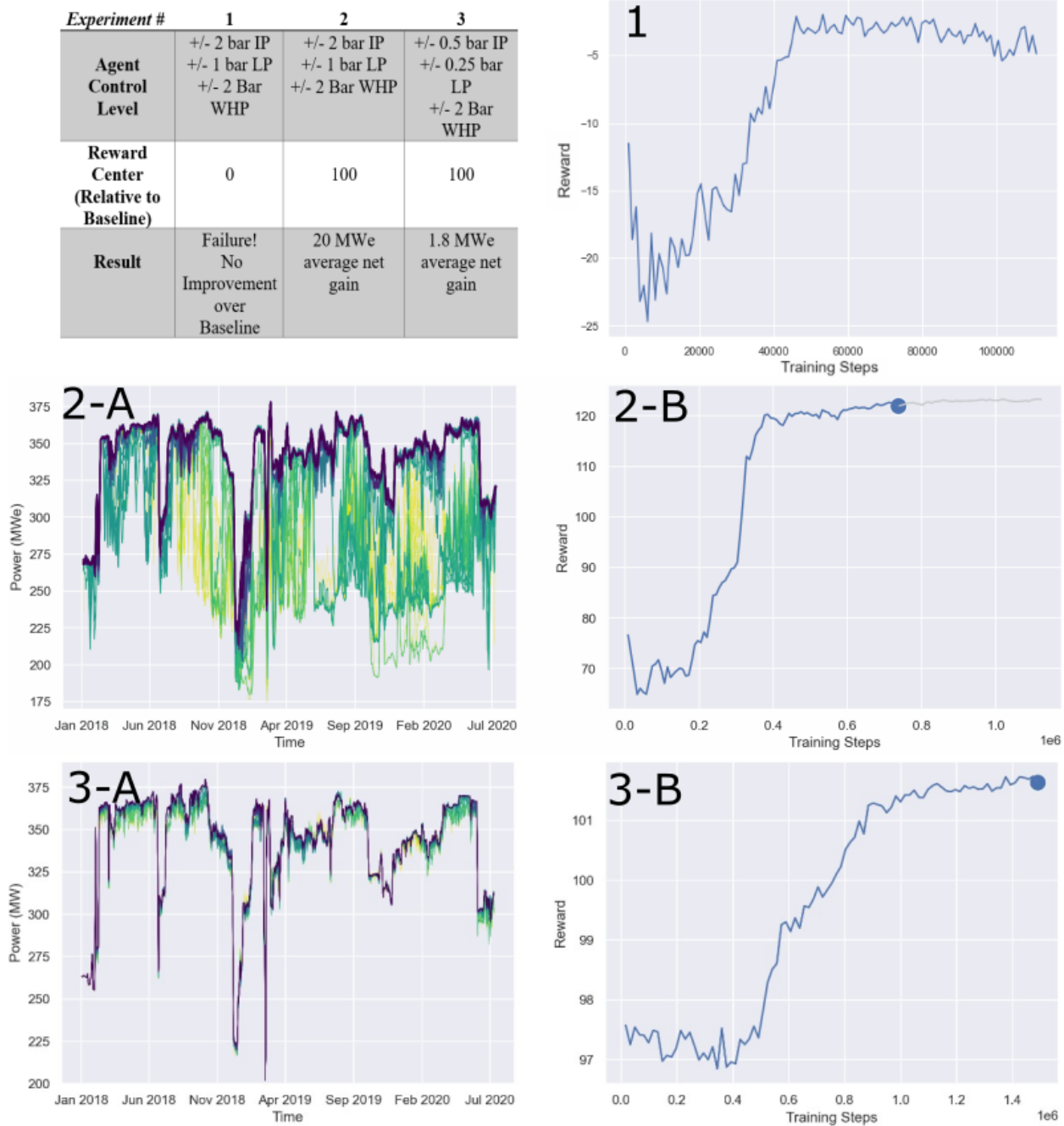
Figure 9: Results of Reinforcement Learning Experiments. Experiment 1 was not successful and was unable to achieve a greater overall output as the reward was set too low. Experiments 2 and 3 improved system output through a reward that was centered at 100% of the total baseline output. By aiming to achieve a higher than baseline, the agent was able to successfully achieve an overall higher production from the system.
