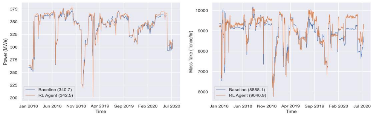
Figure 10: A comparison of our baseline (forecast) model and the RL agent results showing an average increase in power by 1.8 MWe, this resulted in a bit higher mass extraction by 153 tonnes/hour.
