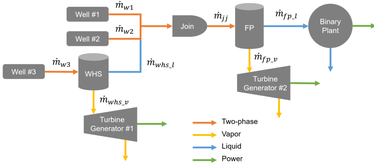
Figure 2: An overview of how components of the GOOML system are connected within a simplified steamfield system network.
