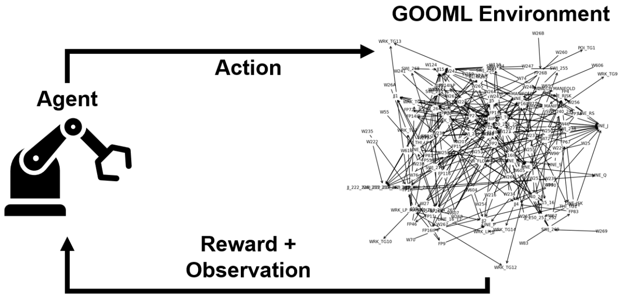
Figure 8: Reinforcement Learning in the GOOML Environment. The agent can take an action in the GOOML environment - here represented by the spaghetti ball - (increase a well flow, throttle a control valve, etc.) and the result yields a reward or a penalty that affects total system power output.
