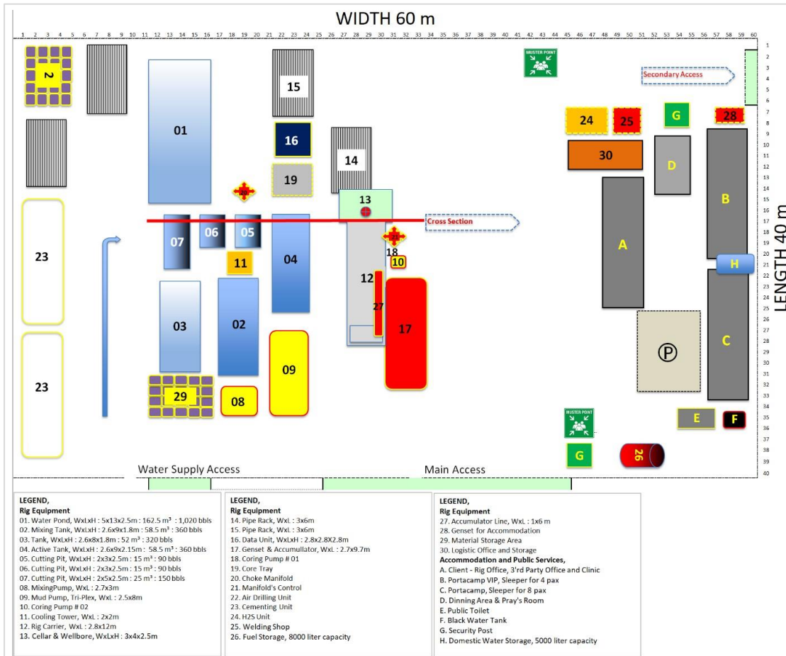
Figure 7. Well-1 pad layout (Sunarso, 2020)
