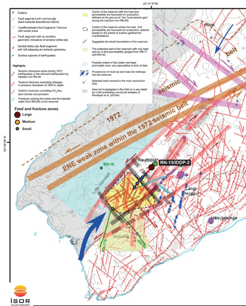
Figure 7: Well path RN-15/IDDP-2 and the location of feed and fracture zones along the path in relation to the tectonic model of the Reykjanes geothermal field (Khodayar et al., 2016a).
