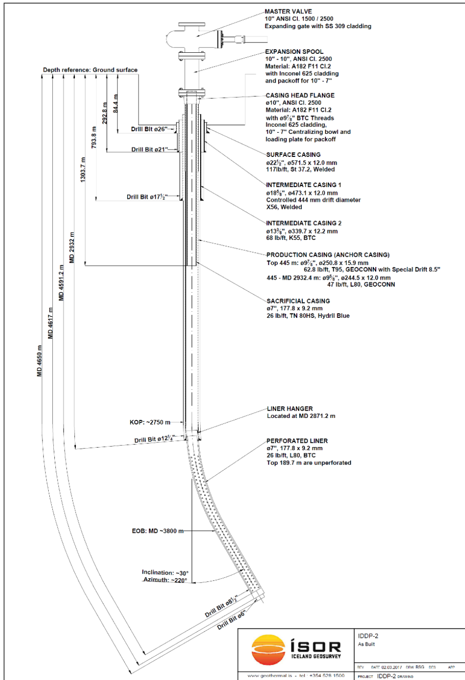
Figure 5: Schematic drawing of well RN-15/IDDP-2 as it was “built”.
