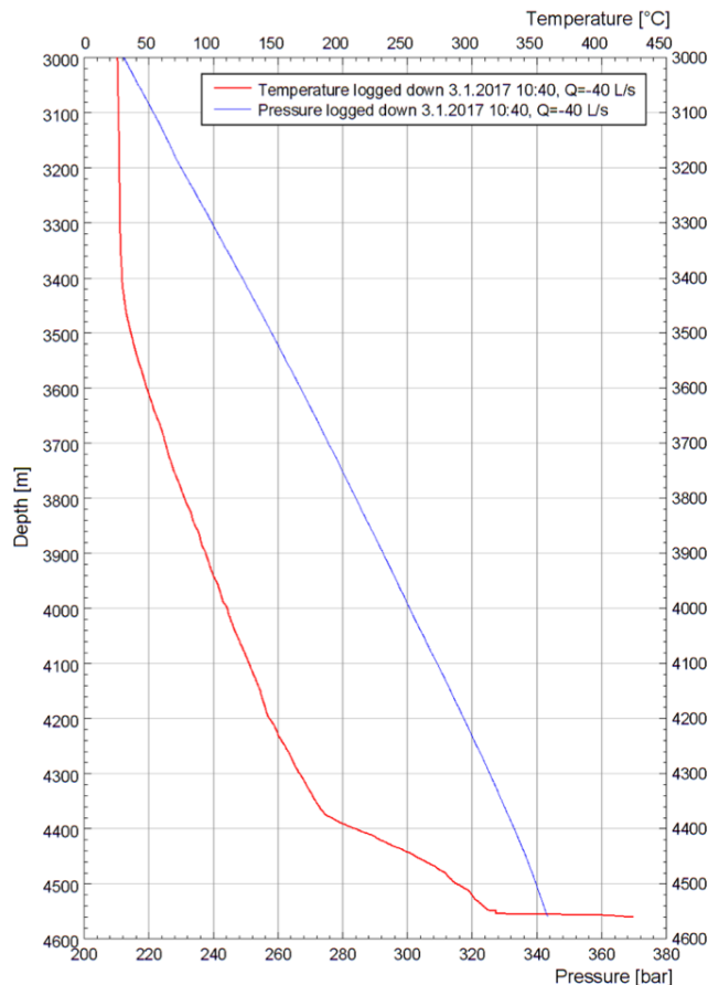
Figure 3: Temperature and pressure logged inside the 7" liner on January 3 rd , 2017.
