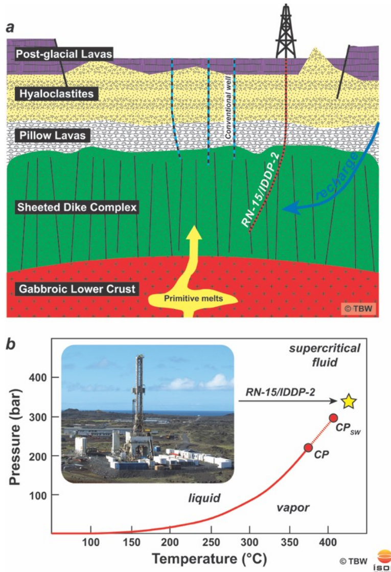
Figure 8: Summary sketch of the RN-15/IDDP-2. a) A simple model that shows the geology of the Reykjanes geothermal system. Sketch is not scaled. b) Temperature-pressure diagram showing the nature of supercritical conditions of the fluids within RN-15/IDDP-2 (CP: critical point; CPSW: critical point of seawater; yellow star: logging results of the temperature-pressure log carried out on January 3 rd , 2017).
