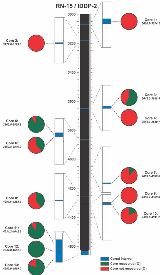
Figure 4: Overview of all core runs conducted in RN-15/IDDP-2. The pie charts provide information about the core recovery (adapted from Weisenberger et al., 2017)
