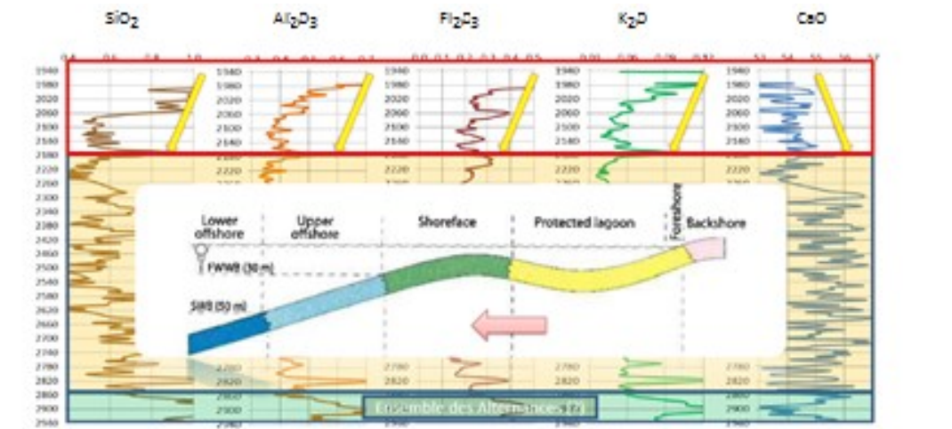
Observed a decrease in the Siliciclastic proxies, related to the different position in the Carbonate platform: from Lagoon to Shoreface
