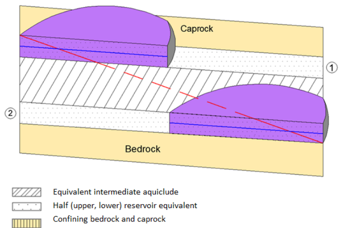
Figure 14.b: Multilayered sandwich equivalent reservoir
