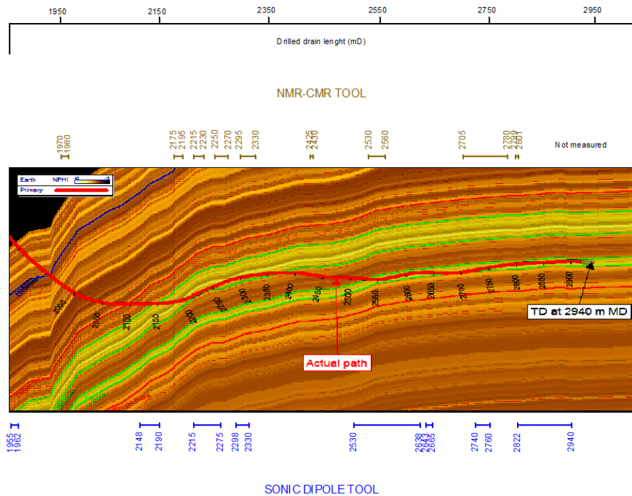
Figure 10: Well GCAH2. Wireline log (NMR-CMC and Sonic Dipole porosity, permeability tools) correlation with drain productive segments
