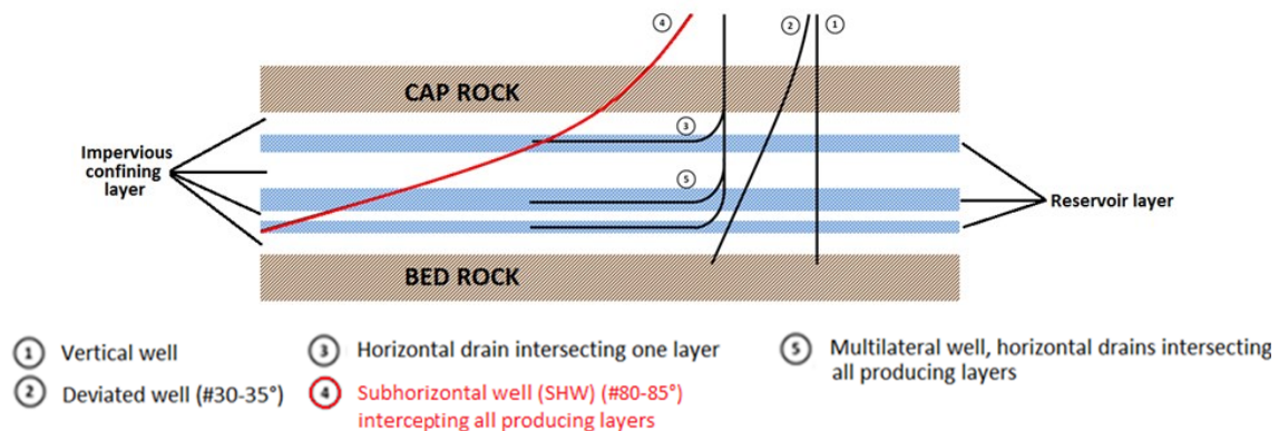
Figure 2: Subhorizontal well concept
