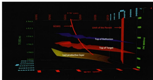
Figure 5: Well GCAH1. Drain trajectory guidelines
