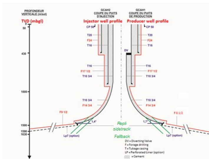
a) Well architectures
