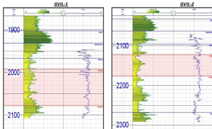
Well GCAH1. Log squaring of nearby offset wells GVIL-1 and GVIL-2
