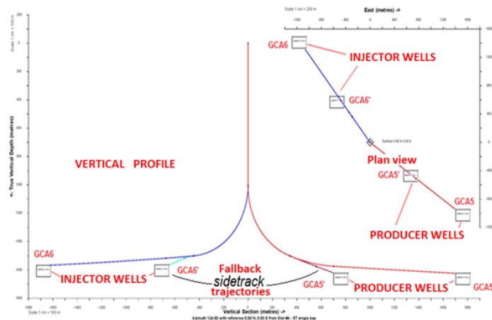
b) Well trajectories
