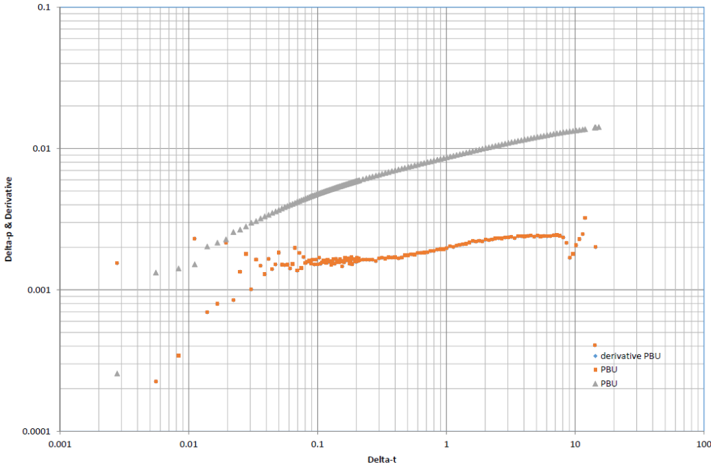
Figure 13: Well GCAH1. Self flowing production test. Build up pressure and derivative log-log plots
