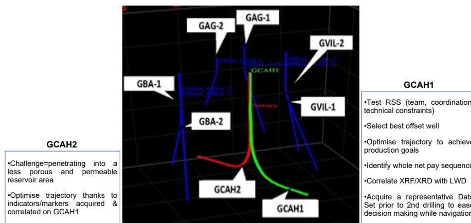
Figure 4: Geosteering strategy and back up from neighbouring offset wells while drilling
