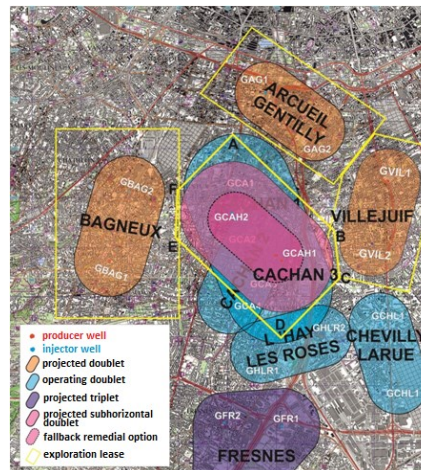
Figure 1: Paris Basin geothermal district heating. Cachan and surrounding locations.
