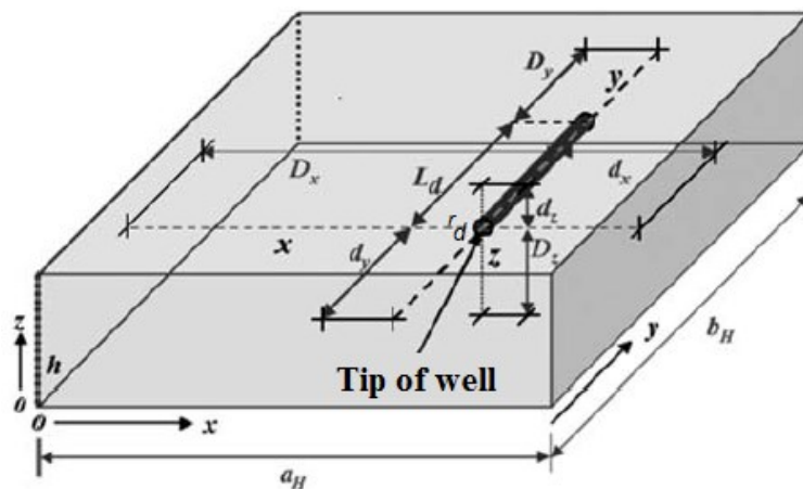
Figure 11 : Well and reservoir geometry for a horizontal well
