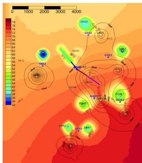
Figure 15: Simulated pressure and temperature patterns (year 2048)
