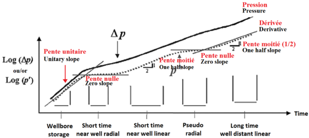
Figure 12: (Sub)horizontal drain (idealised) flow regime identification (after Lee et al, 1982)
