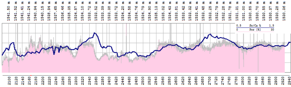
Correlation between raw Porosity log and Sr/Ca
