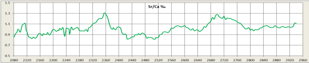
Sr/Ca plot highlighting the (0.7-1.1%) interval
