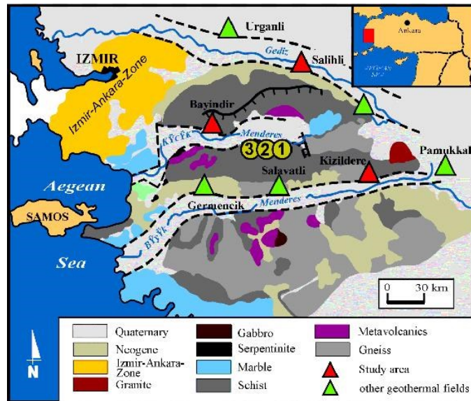
Fig. 1. Geologic setting of the Menderes massif with some locations of active geothermal waters and some locations of epithermal mineralizations as extinct geothermal systems (1: Hg deposit; 2: Sb deposit; 3: Au deposit; Özgür, 1998).
