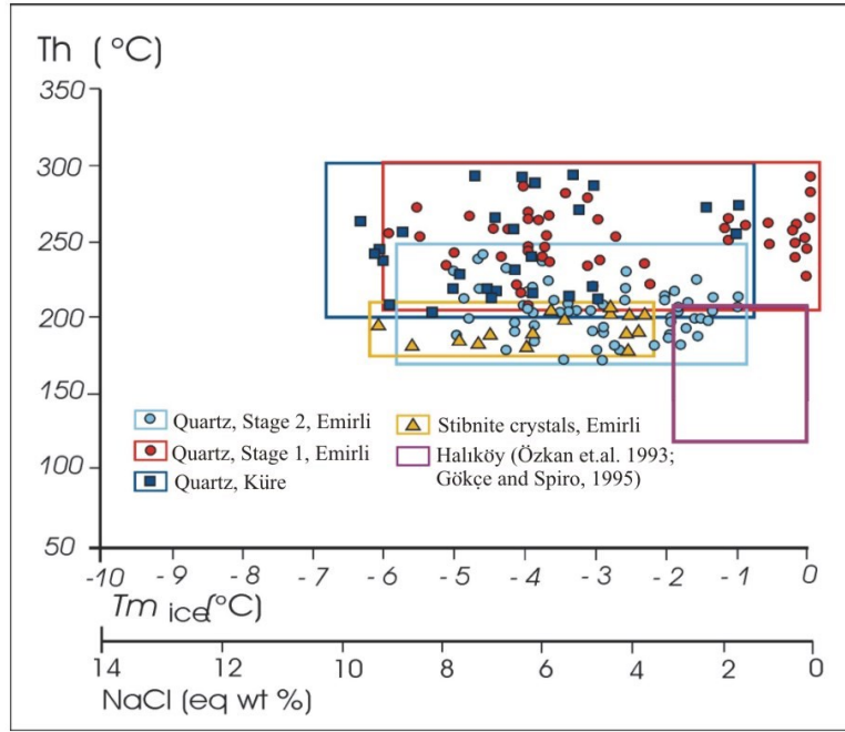
Fig. 3. Homogenization temperatures, salinity and T_{m\text{ice}} in quartz and stibnite crystals of Hg, Sb and Au deposits of Haliköy, Emirli and Küre in the continental rift zone of the Küçük Menderes within the Menderes Massif (Özgür, 1998, 2019).
