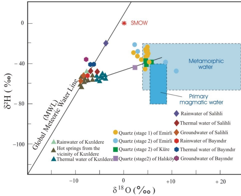
Fig. 4. Plot of \delta^{18}\text{O} versus \delta^2\text{H} in epithermal fluids of quartz crystals of ore fields of Halıköy, Emirli and Küre and active geothermal waters of Kızıldere, Bayındır and Salihli as well (Özgür, 1998).
