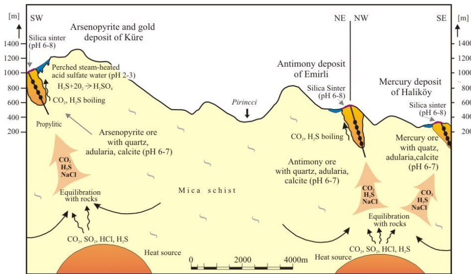
Fig. 6. Simplified genetical modeling of Hg, Sb and Au mineralizations of Haliköy, Emirli and Küre in the continental rift zone of the Küçük Menderes within the Menderes Massif (Özgür, 1998, 2019).
