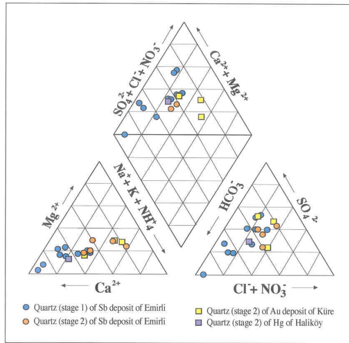
Fig. 5. Hydrogeochemical classification of fluids of the Hg, Sb and Au ore fields of Halıköy, Emirli and Küre (Özgür, 1999).
