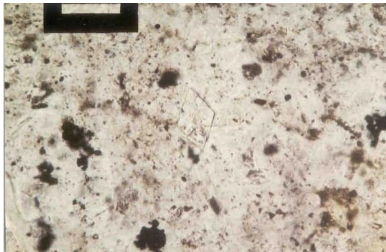
Fig. 7. Microscopical observation of rhomboidal, triclinic adularia crystals in strong silicified host rocks of Sb mineralization of Kuşunlu in the continental rift zone of the Gediz within the Menderes Massif. 500 X and // N (Özgür, 1998, 2019).
