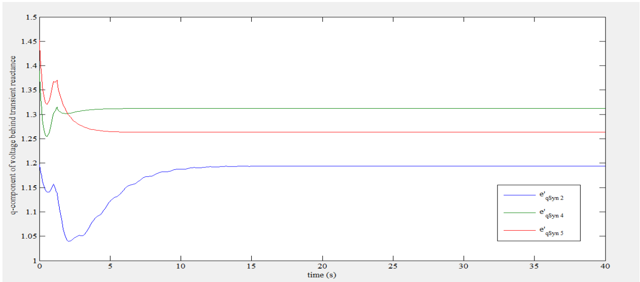
Figure 3.6 q-axis voltage component behind transient reactance responses with UPFC
