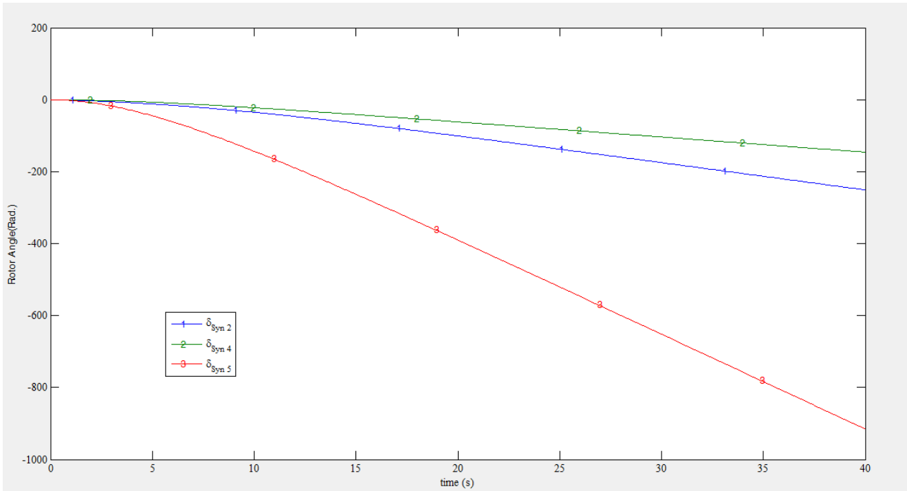
Figure 3.4: Rotor angle responses with IPFC FACTS device, Fault applied at Bus 04
