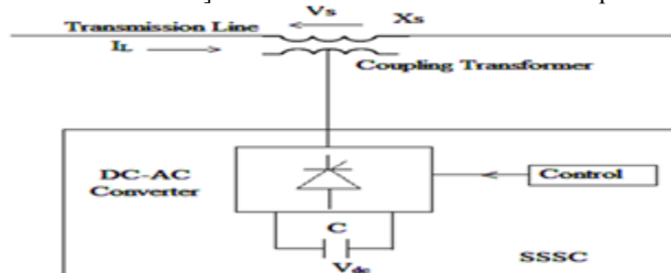
Figure 2.2: Voltage source model of SSSC
