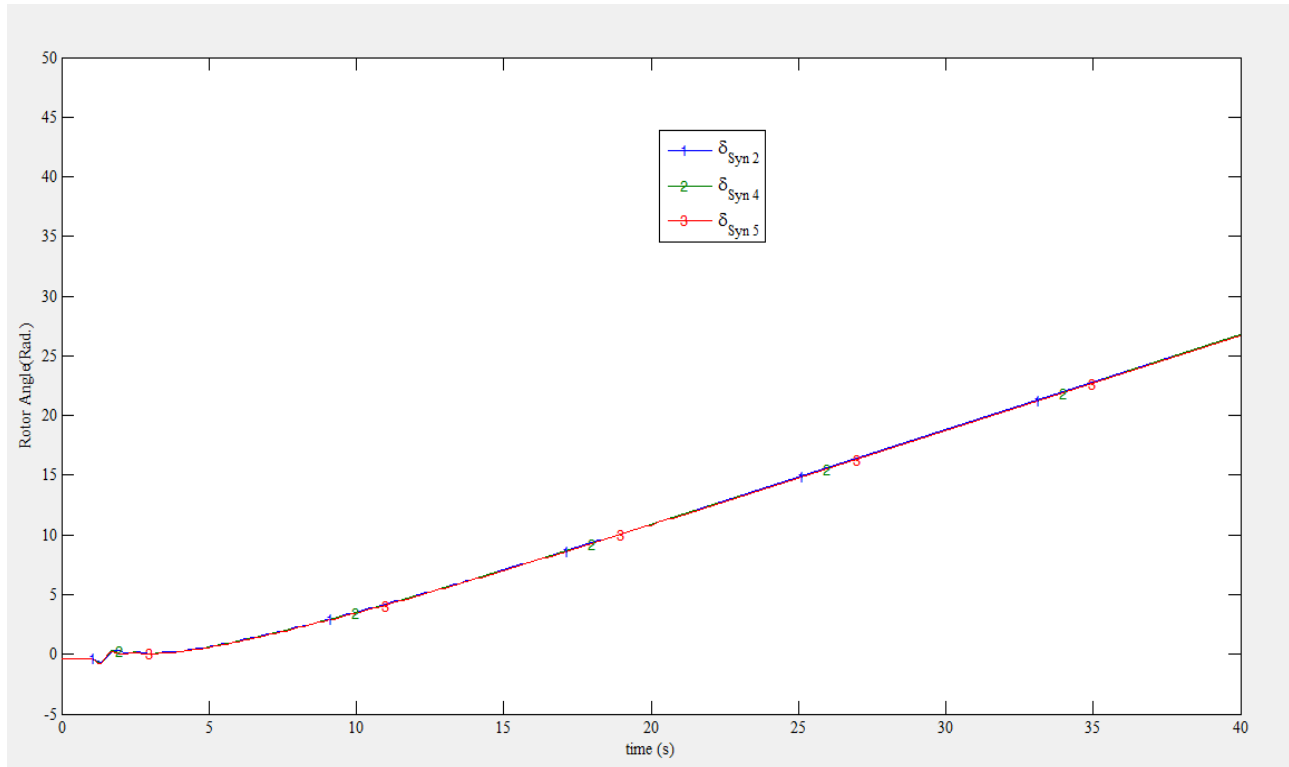
Figure 3.1: Rotor angle responses without FACTS, Fault at Bus 04
