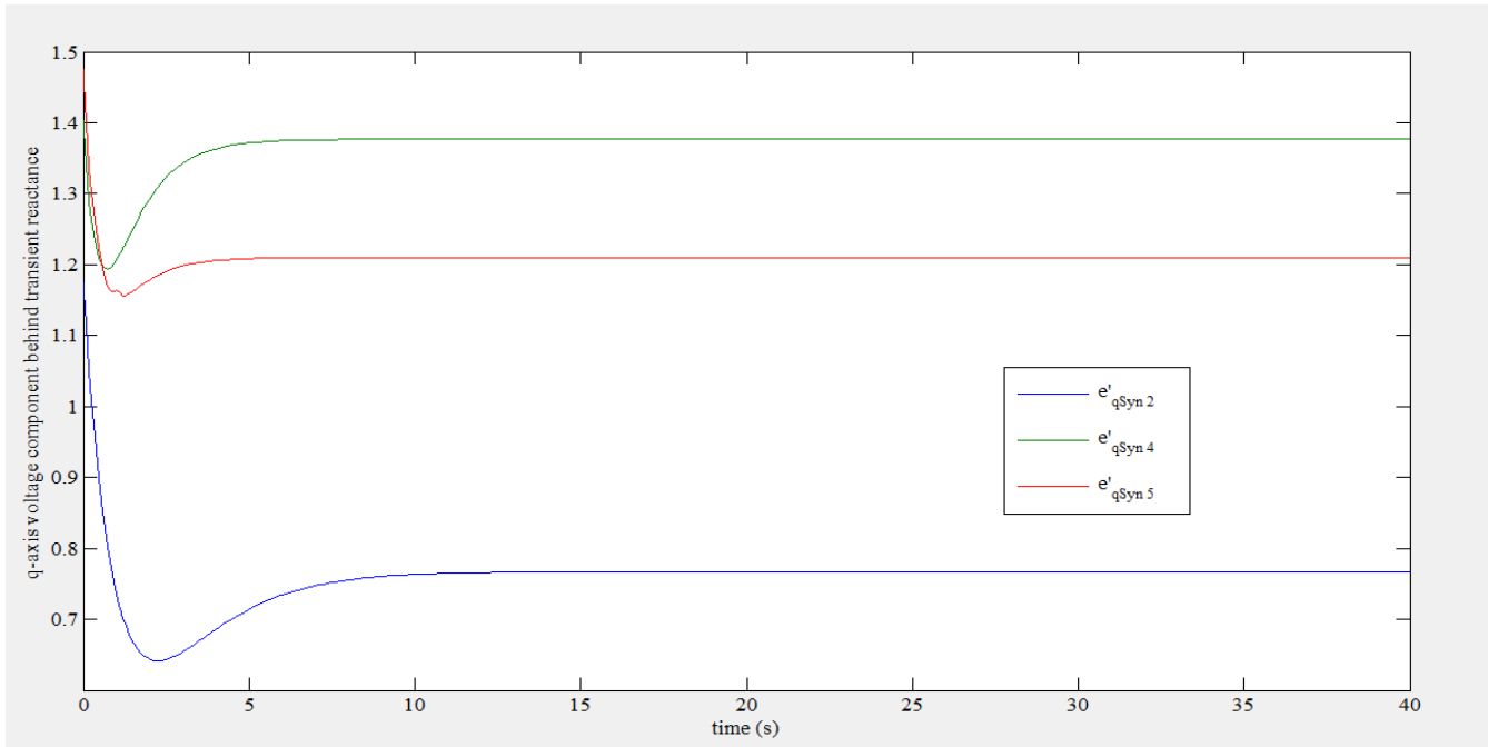
Figure 3.8: q-axis voltage component behind transient reactance responses with IPFC
