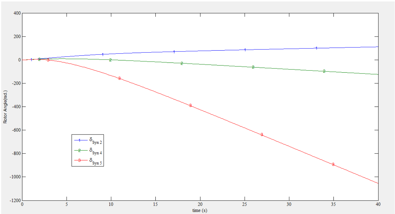
Figure 3.3: Rotor angle responses for SSSC FACTS device, fault applied at Bus 04
