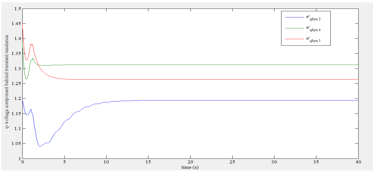
Figure 3.7: q-axis voltage component behind transient reactance responses with SSSC
