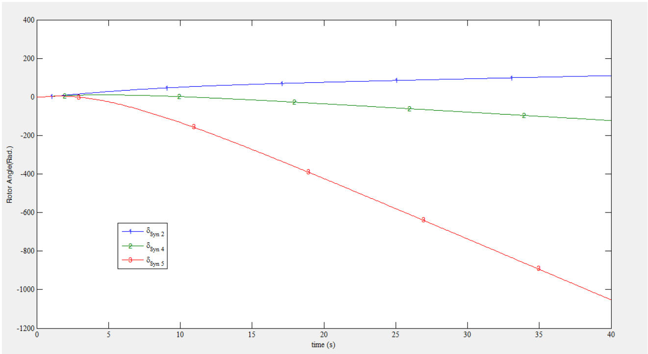
Figure 3.2: Rotor angle responses UPFC FACTS device, fault applied at Bus 04
