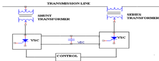
Fig 2.1: UPFC VSC model
