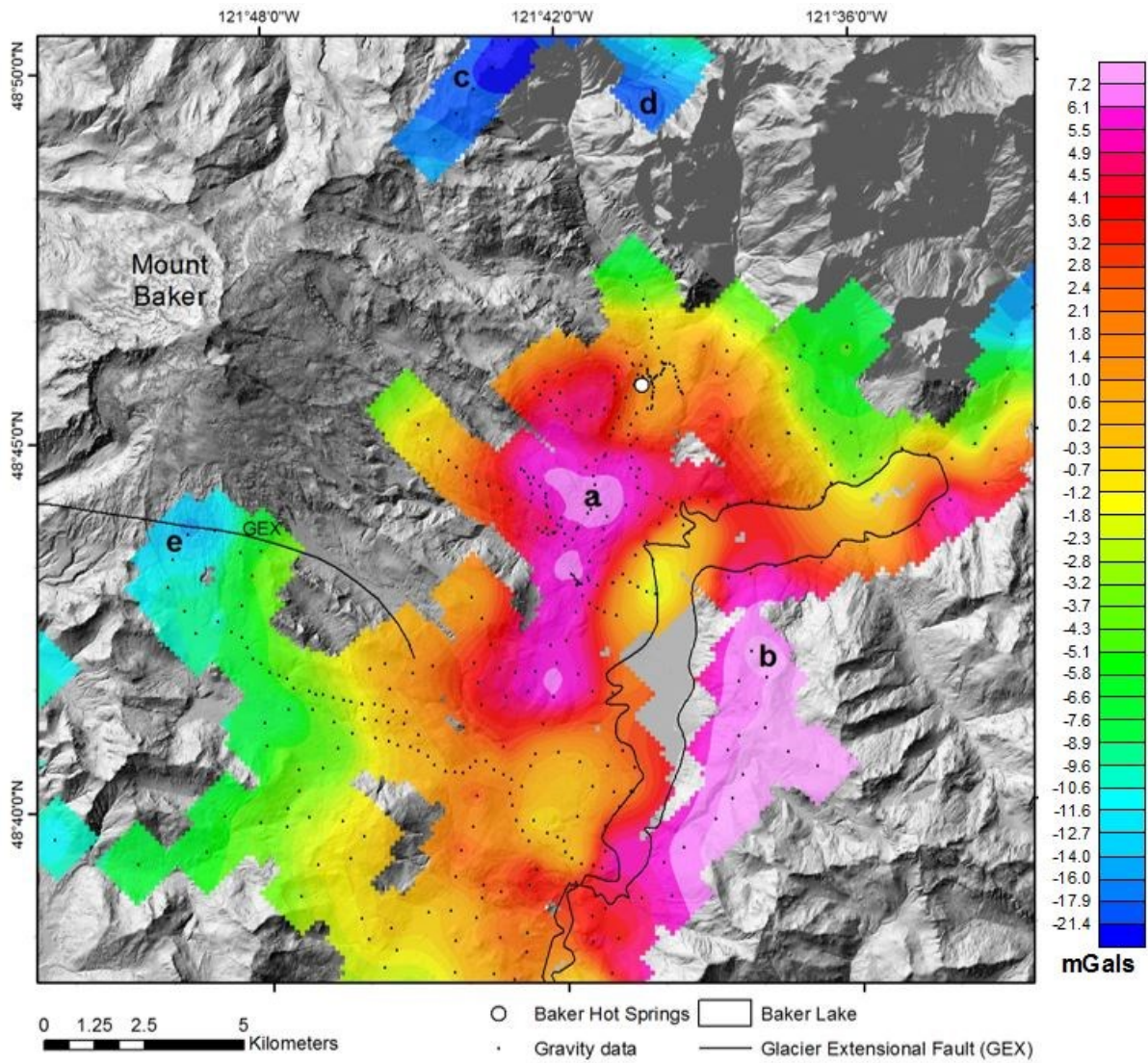
Figure 6. Isostatic gravity anomaly map produced from Phase II survey data. Key features labeled a-e.
