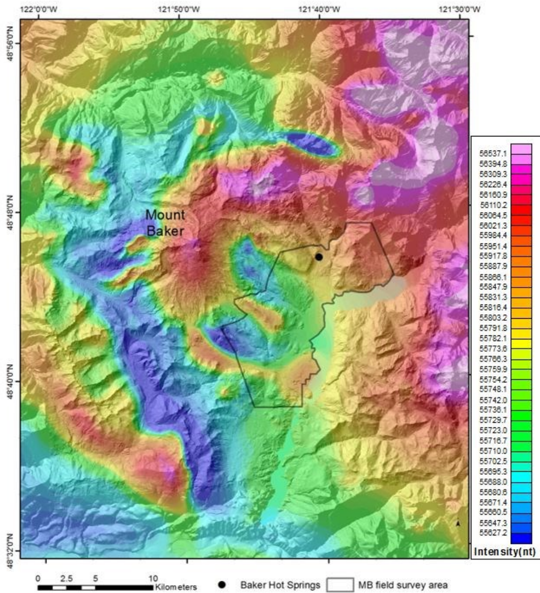
Figure 4. Regional Aeromagnetic map of the Mount Baker Survey Area and surrounding region.
