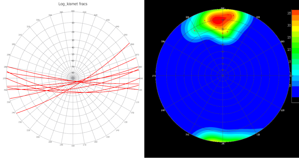
Figure 7: Stereographic projections of hydraulic fractures at the kISMET site. Left: plane plot. Right: contoured pole plot.
