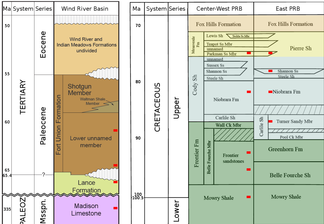
Figure 3: The relevant stratigraphy of the WRB and PRB spanning from Paleocene to Mississippian, and Upper to Lower Cretaceous. Approximate sample location-ages are marked with red boxes. Note that WRB samples vary mainly by depth, and PRB samples vary laterally.
