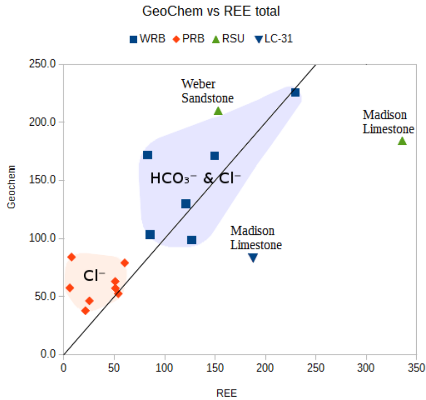
Figure 6: A graph of the result of applying our first attempt at a formulaic relationship between ligands and total REEs. The good fit of the present relationship is mostly due to the abundance of bicarbonate in the WRB (blue), which allows those data to be fit independently of the chloride-dominated PRB (orange). The two green data points are from an early study by our team of the Rock Springs Uplift (McLing et al., 2014).
