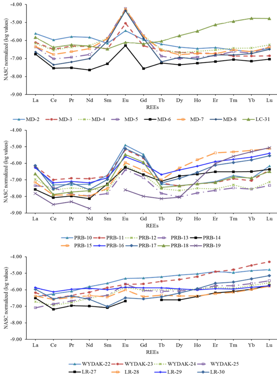
Figure 5: Three NASC-normalized REE diagrams for the WRB, PRB, and power stations in this study. a) The WRB samples come from clastic sandstone reservoirs except for sample LC-31 which comes from a deep carbonate reservoir. b) The PRB samples generally come from rocks of marine genesis, and the high Gd signature of the reservoir transfers to the water. The samples with the greatest HREE concentration come from the field on the axis of the basin. c) The power station samples come from ponds subject to different evaporation ratios, except WYDAK-25 which came from a truck used to collect fly-ash washed off of the scrubber.
