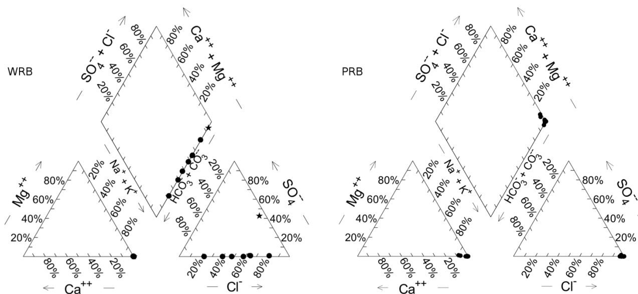
Figure 4: Piper diagrams for the WRB and PRB waters in this study. The PRB is dominated by \text{Na}^+ and \text{Cl}^- but many samples in the WRB have substantial bicarbonate. The star represents the reject brine of the water treatment plant, which unlike all other samples contains significant sulfate as a result of engineered processes.
