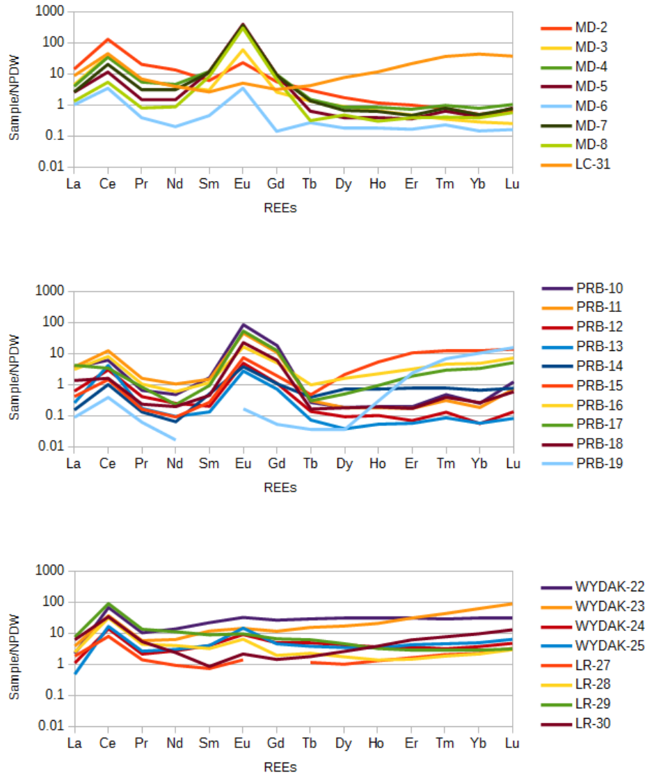
Figure 5: Three NPDW-normalized REE diagrams for the WRB, PRB, and power stations in this study. a) The WRB samples contain more LREEs and Eu than the oceans, but lower HREEs. b) The PRB samples contain more Eu and Gd than the oceans and in some cases more HREEs c) The power station samples are generally flat, indicating similarity to ocean water, but have a marked HREE enrichment and the highest concentrations of the critical REEs Tb, Dy, and Er found in this study.
