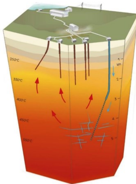
Figure 1: A conceptual model showing the EGS system in the Reykjanes field (Friedleifsson et al., 2016)
