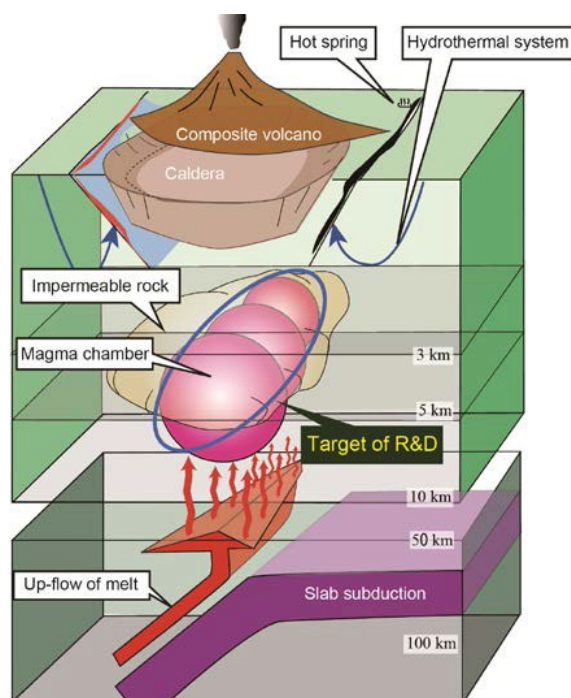
Figure 2: Conceptual model for supercritical geothermal systems in northern Honshu, Japan (Asanuma et al., 2015). These systems lie above shallow magma chambers that are associated with Miocene and younger caldera complexes in the Tohoku region.
