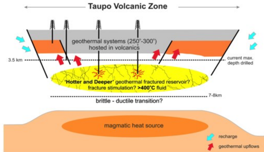
Figure 3: Conceptual model for the HADES project (from Bignall and Carey, 2011, after Heise et al., 2007)
