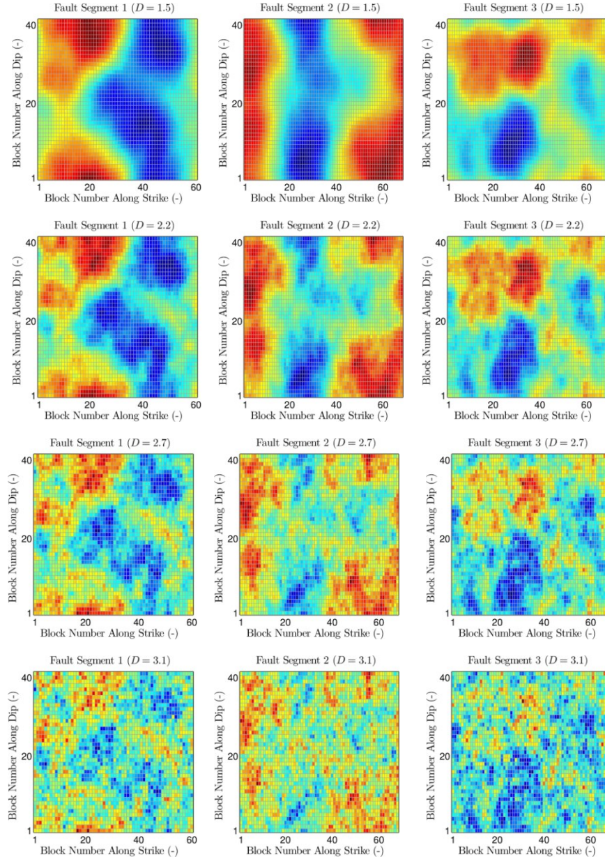
Figure 11: Heterogeneity patterns across each en-echelon fault segment in the numerical model.
