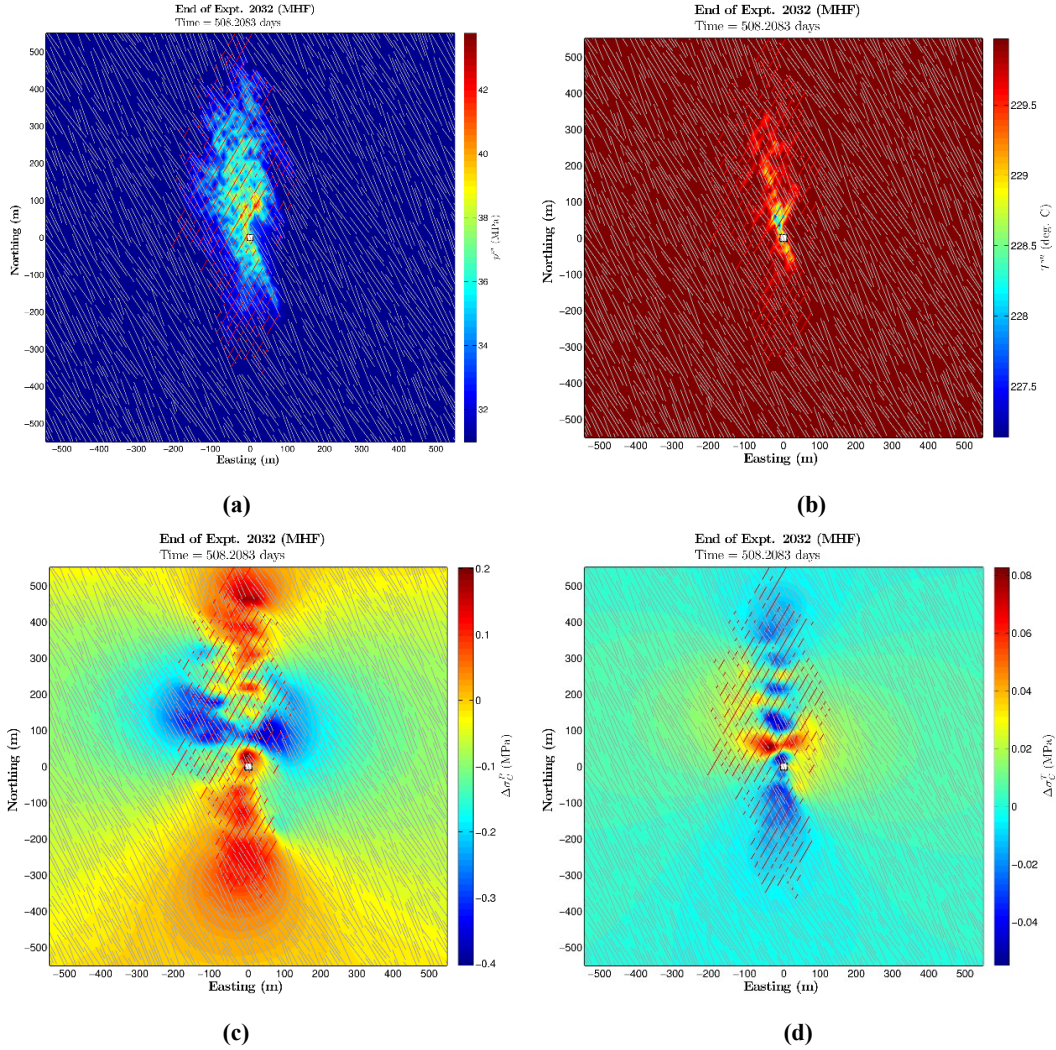
Figure 7: Distribution of (a) matrix fluid pressure, (b) matrix temperature, (c) change in Coulomb stress caused by poroelastic effects, and (d) change in Coulomb stress caused by thermal effects at the end of Expt. 2032 (MHF) for Case D.
