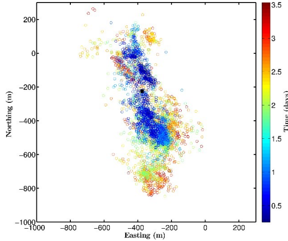
Figure 2: Microearthquake locations recorded during the Expt. 2032 (MHF) stimulation treatment at Fenton Hill colored by event timing. The well was shut-in after roughly 2.5 days.
