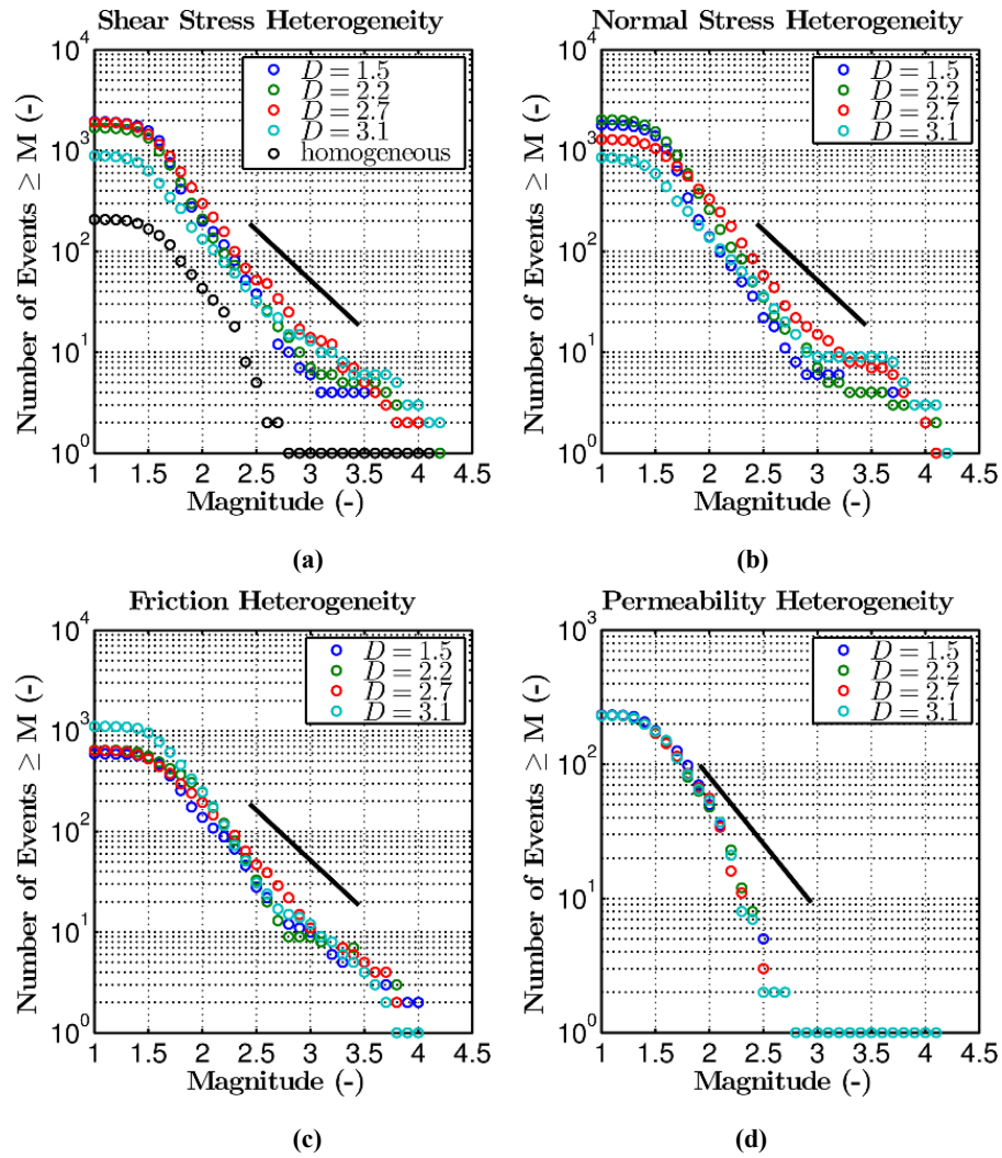
Figure 13: Simulated frequency-magnitude distributions for the low stress drop case (Case F). The solid black line represents a GR b-value of one.
