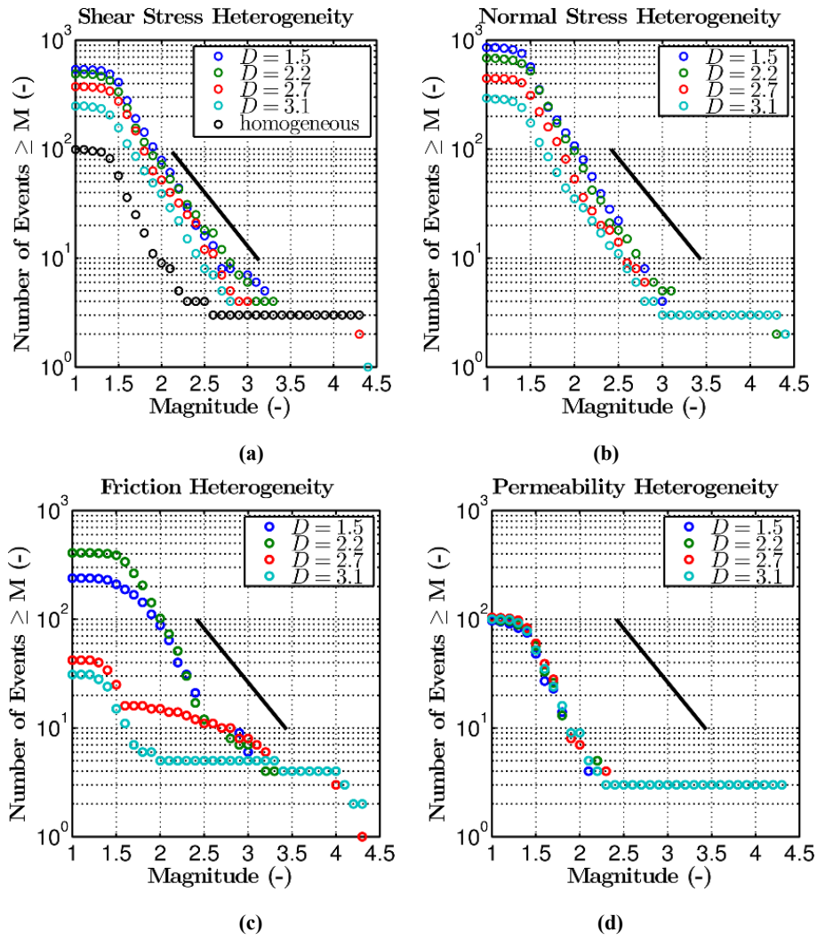
Figure 12: Simulated frequency-magnitude distributions for the large stress drop case (Case E). The solid black line represents a GR b-value of one.
