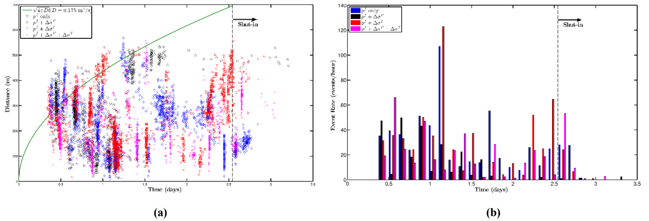
Figure 6: Comparison of (a) distance from well and (b) event rate for Cases A – D during Expt. 2032.
