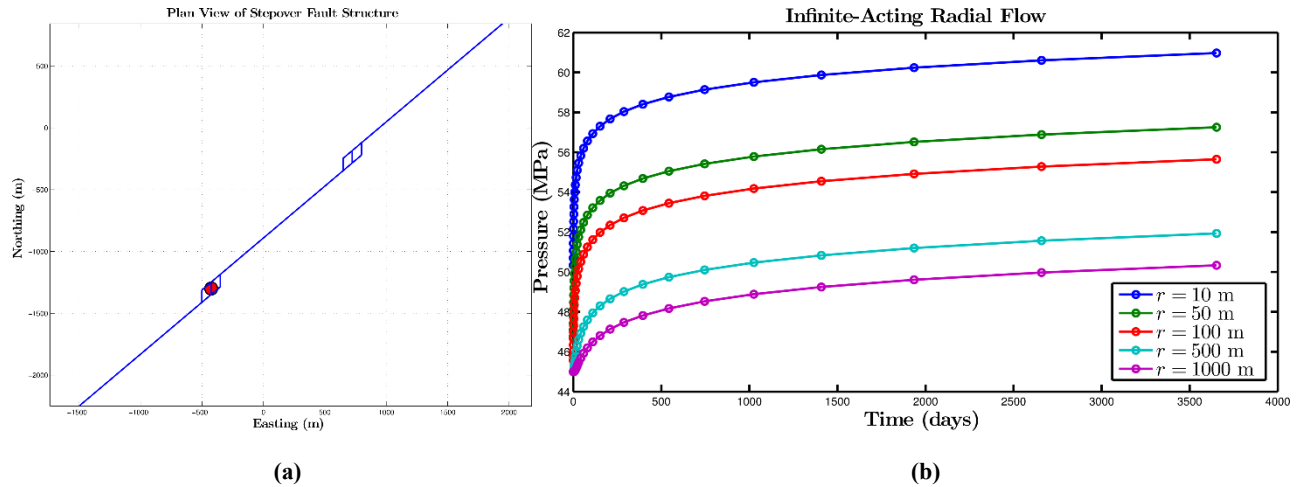
Figure 10: (a) Plan view of the en-echelon stepover fault model geometry, and (b) infinite-acting radial flow (IARF) solution for injection into an aquifer of finite thickness and. The hydraulic connection between the well and the basement fault was assumed to occur at one of the stepover features and modeled as a time-dependent pressure boundary condition based on the IARF solution at a distance of 100 m from the well.
