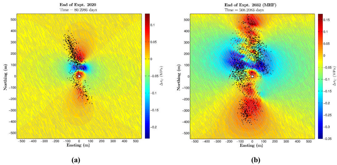
Figure 8: Contours of total change in Coulomb stress (a) at the end of Expt. 2020 and (b) at the end of Expt. 2032. The black dots represent microearthquake event locations that occurred during each of the stimulation treatments.
