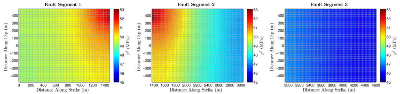
Figure 14: Pressure distribution along fault for Case E4 (fractal dimension 2.7) after 422 days of injection.
