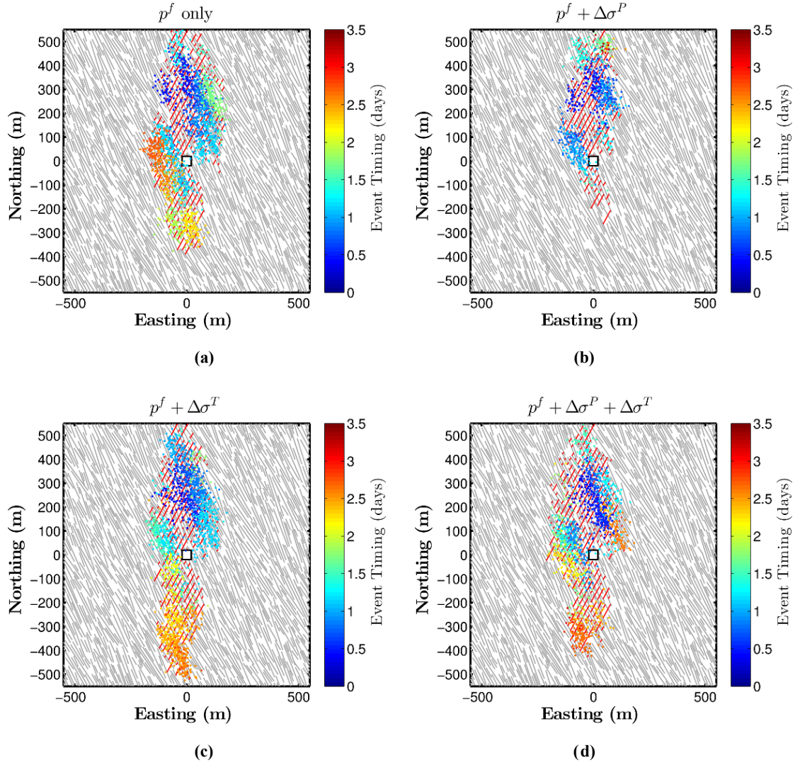
Figure 5: Stimulated fracture network and microseismic event locations at the end of Expt. 2032 (MHF) for (a) Case A, (b) Case B, (c), Case C, and (d), Case D. The red lines are hydraulic splay fractures generated during the stimulation treatment.
