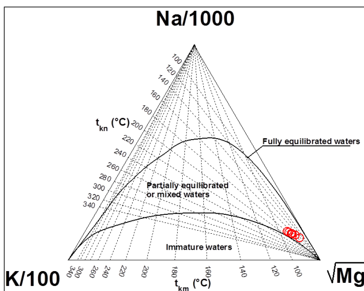
Figure 5. Na-K-Mg ternary diagram for waters collected from Lojing area, Kelantan.
