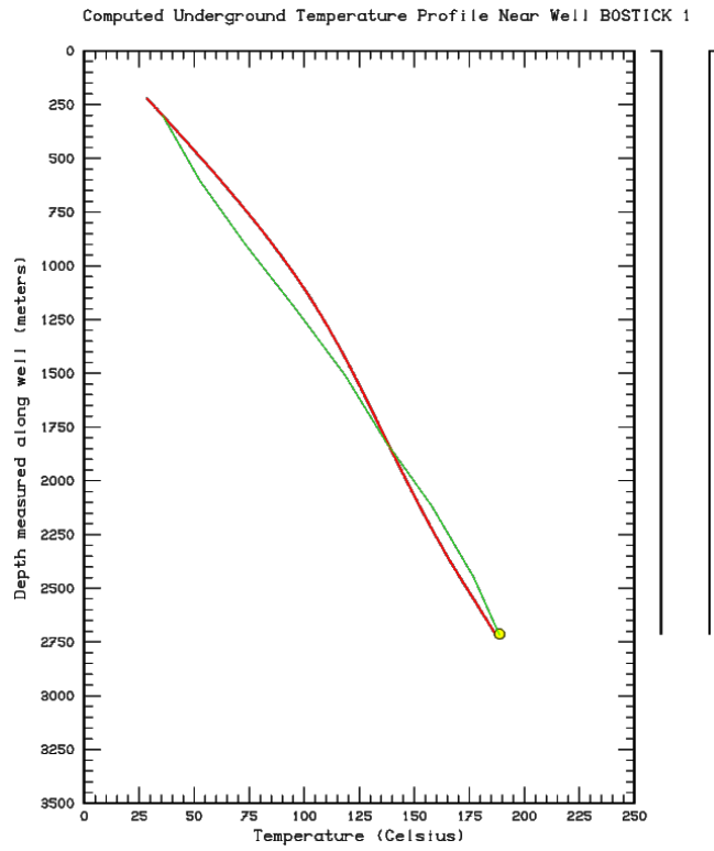
Figure 6: Comparison between computed (solid red line) and measured temperature profiles (solid green line and yellow circle) for well Bostick1. No information is available concerning the shut-in time at which the temperature survey was taken.
