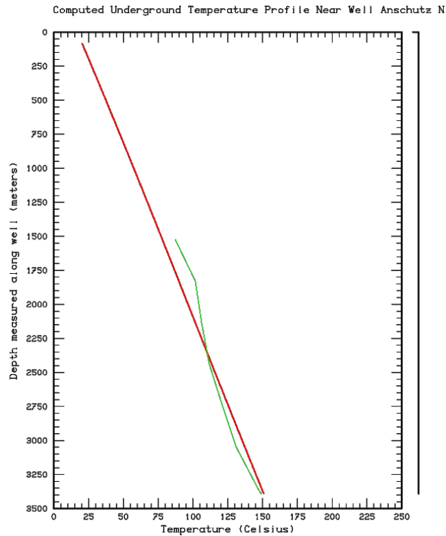
Figure 10: Comparison between computed (solid red line) and measured temperature profiles (solid green line) for well Anschutz No. 1. The temperature survey was taken after the well had been shut-in for about 66 hours.
