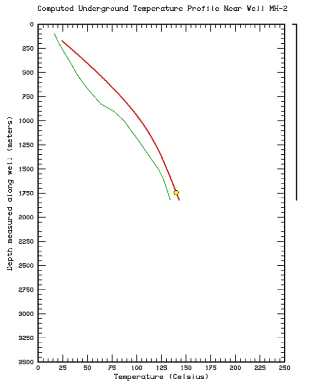
Figure 9: Comparison between computed (solid red line) and measured temperature profiles (solid green line) for well MH-2. Survey was run 76 days following completion of drilling. The yellow circle is the measured flowing temperature at this depth. Since the measured flowing temperature is higher than the recorded shut-in temperature (solid green line), it is almost certain that the shut-in survey does not represent the stable formation temperatures.
