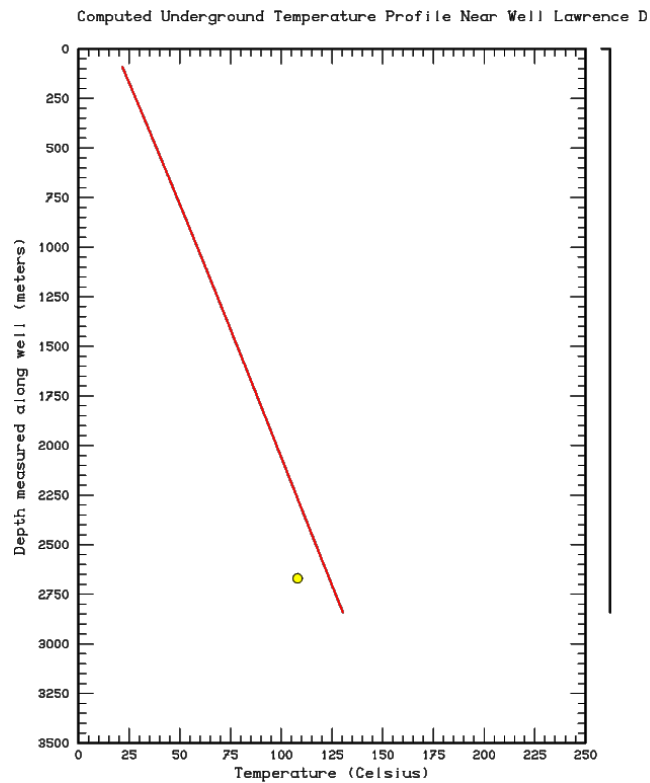
Figure 8: Comparison between computed (solid red line) and measured temperature profiles (yellow circle) for well Lawrence D No. 1. The measured temperature was recorded after the well had been shut-in for only about 8 hours.
