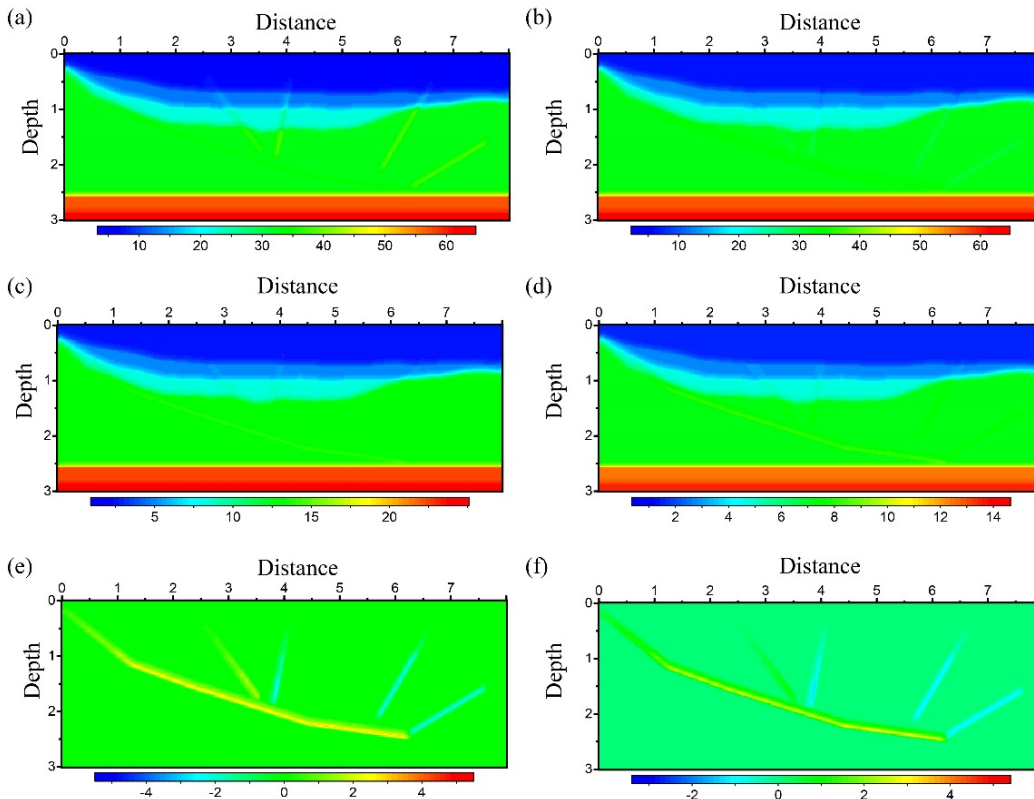
Figure 2: Initial models for AEWI obtained by smoothing those in Fig. 1: (a) C_{11} , (b) C_{33} , (c) C_{55} , (d) C_{13} , (e) C_{15} , and (f) C_{35} . Unit is GPa.
