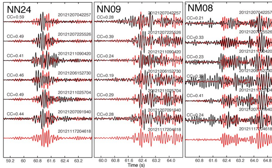
Figure 6: Three different stations showing the seismic signal of six different events found indirectly linked (black traces) to reference event 47 (red traces).
