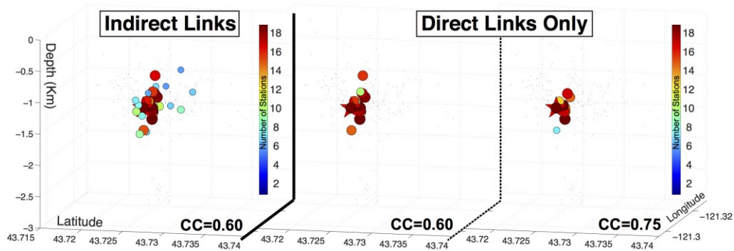
Figure 4: Comparison between results including both direct and indirect linked events (left) for a threshold of CC=0.6 and including only directly linked events (middle and right) for detection thresholds of CC=0.6 and CC=0.75 . Again, color and size represent the number of stations that link the event to reference event 47. Warmer colors and larger size both represent a larger number of stations as indicated in the color bar. The red star represents the reference event (high PageRank).
