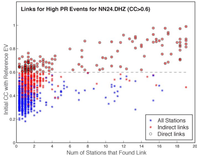
Figure 5: CC at station NN24 vs. number of stations linking the event to the reference event. Direct links (red stars with black circles), indirect links at station NN24 (red star), indirect link at other stations (blue stars).
