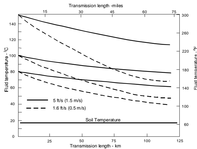
Figure 3. Temperature drop in hot water transmission line (Ryan 1981)
