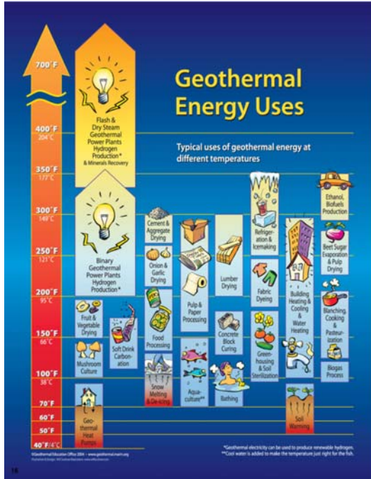
Figure 1. Various geothermal uses, including power generation and direct-use, related to their appropriate temperature range (courtesy of Geothermal Education Office)
