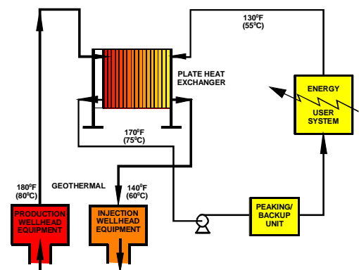
Figure 2. Typical direct-use geothermal heating system configuration
