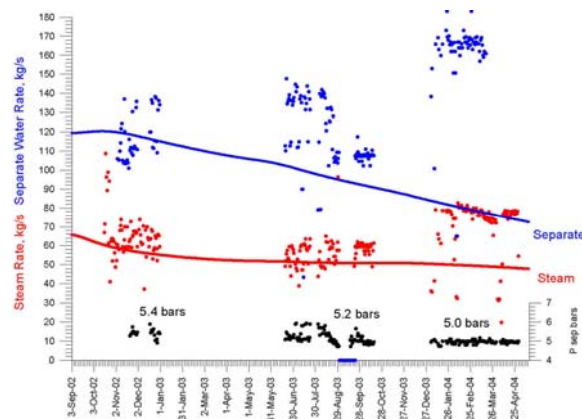
Figure. 9. Model matches (scenario #3): modeling steam and separate production from wells 016, 26, E4, 029W, E5 (referenced to 5.2 separation pressure, ati) against total PP production during exploitation of the Dachny site. Dots – PP exploitation data (Fig.6), solid line – modeling results.
