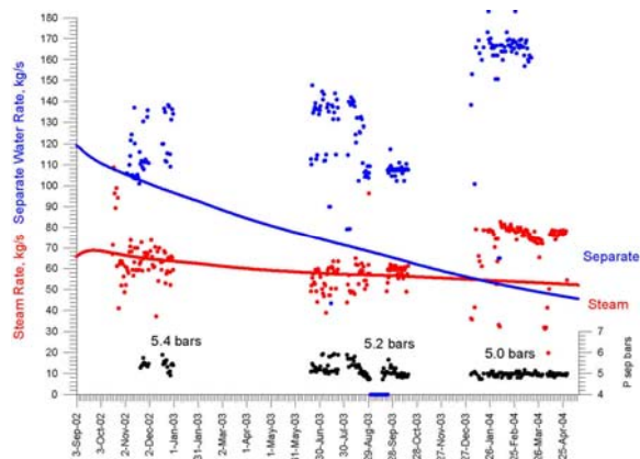
Figure. 8. Model match (scenario #2): modeling steam and separate production from wells 016, 26, E4, 029W, E5 (referenced to 5.2 separation pressure, ati) against total PP production during exploitation of the Dachny site. Dots – PP exploitation data (Fig.6), solid line – modeling results.
