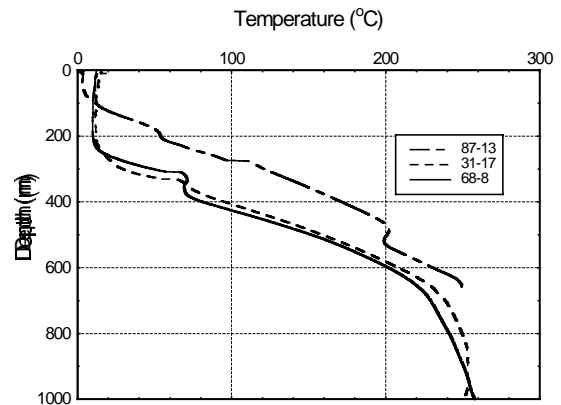
Figure 2. Temperature profiles for the upper 1000 m of the three wells discussed in the text.
