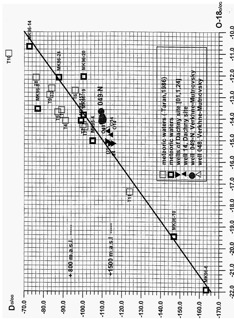
Fig.2 D & O18 distribution in flims of Mutnovsky geothermal field.
