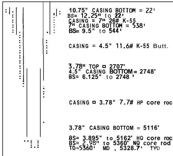
Fig. 3. Newberry well 76-15TCH.
