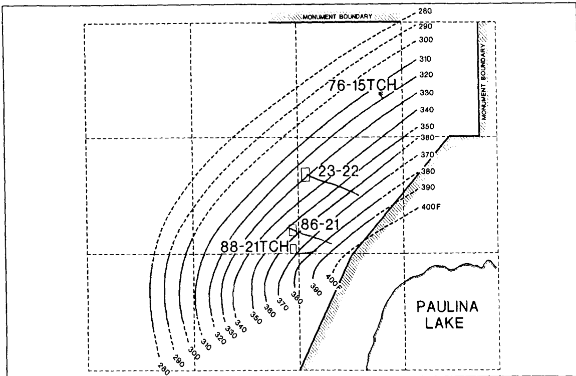
Fig. 1. Plan view of Newberry project area, with temperature isotherms at 2000 ft ASL
