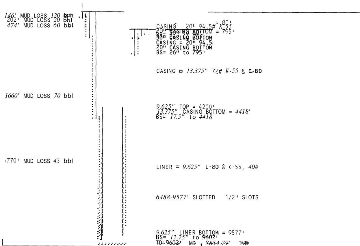
Fig. 5. Newberry well 23-22
