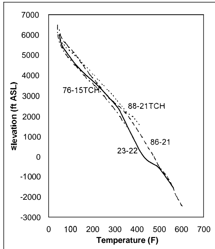
Fig. 6. Newberry temperature profiles.
