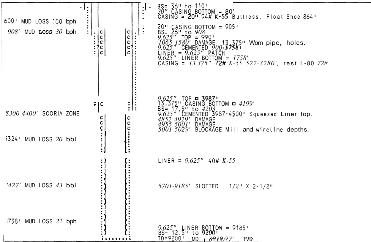
Fig. 4. Newberry well 86-21.
