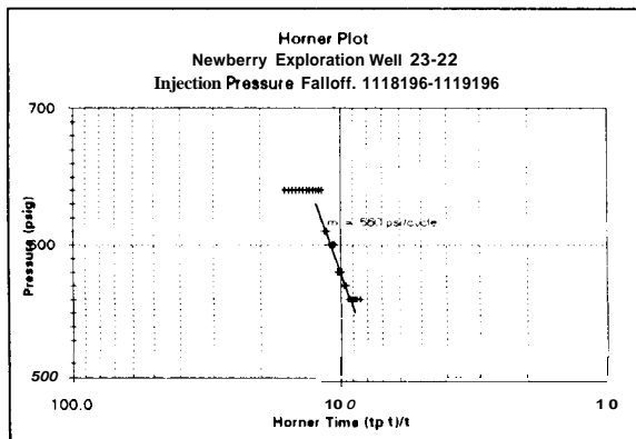
Fig. 7. Injection falloff analysis.
