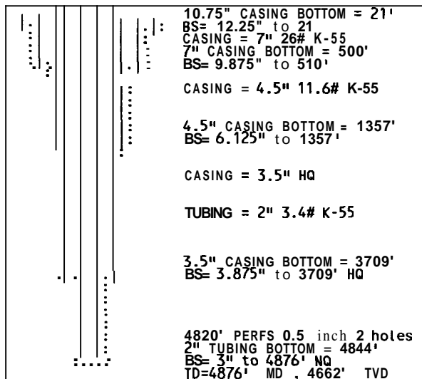
Fig. 2. Newberry well 88-21TCH.
